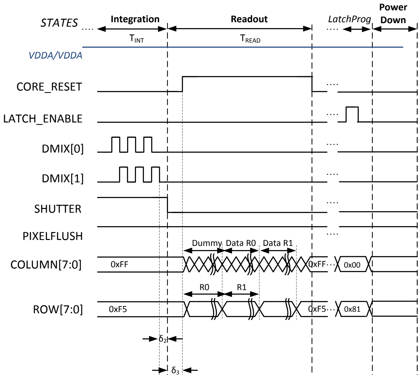
Figure 12: Global timing diagram from integration to power down. Each phase consists of a reset period, an integration period and a read-out phase. The last LatchProg phase here is used to put the sensor in Power Down mode.
