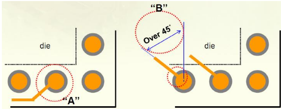
Figure 22: Recommended trace layout
