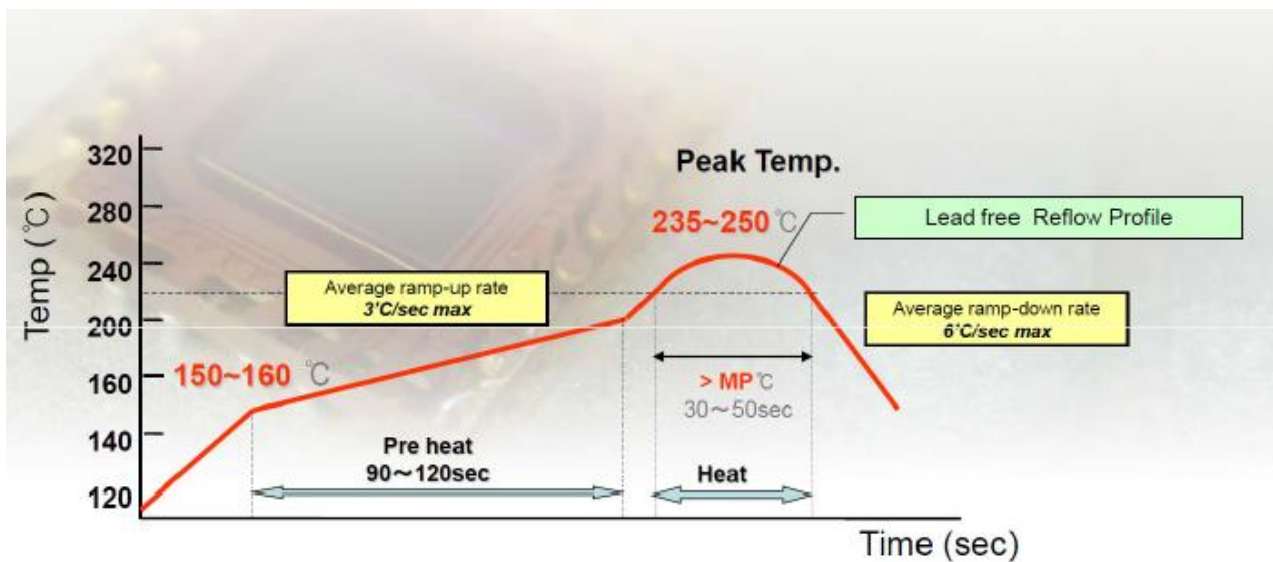
Figure 23: Recommended reflow profile
