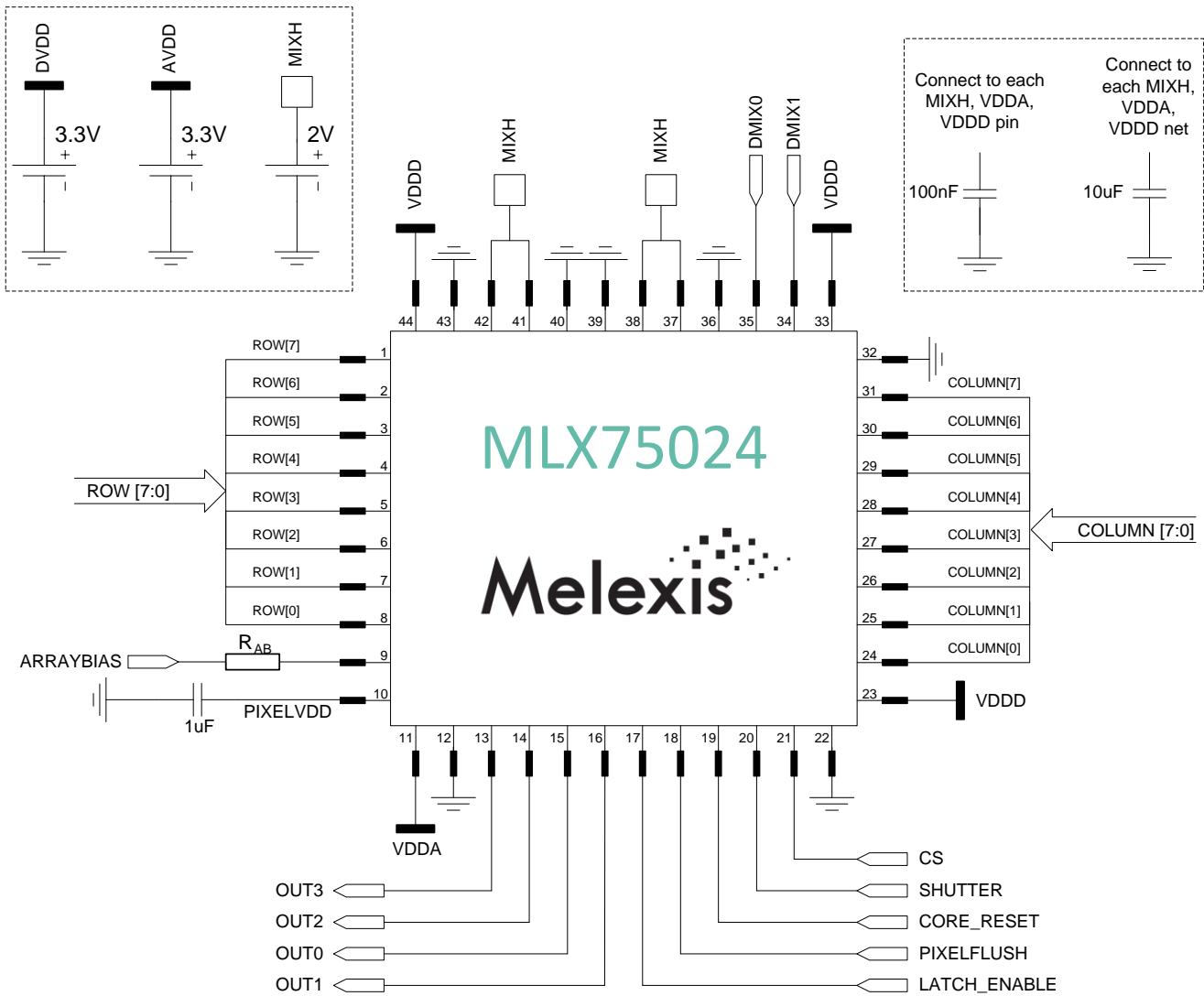
Figure 4: Typical connection diagram 3
