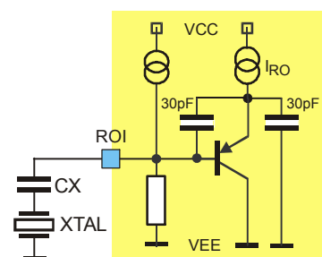
Fig.7: RO schematic
