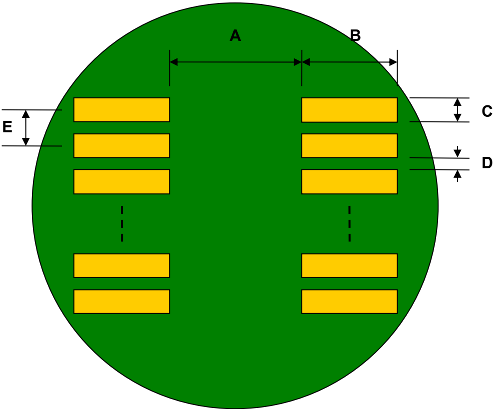
Top View (SMT Footprint)
