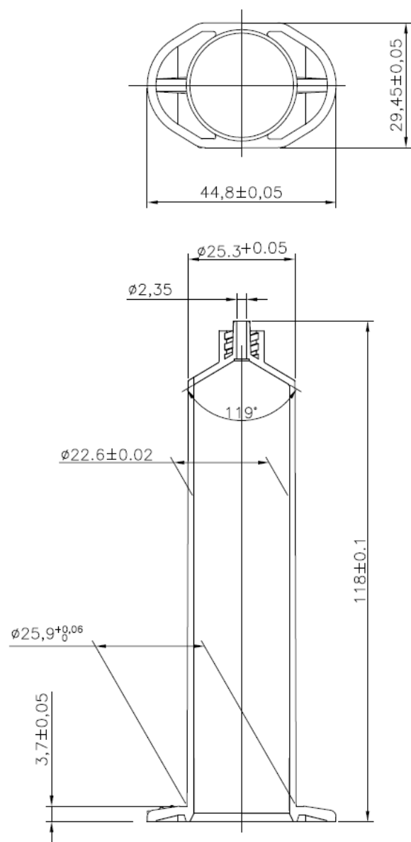
Image 1: 30cc syringe dimensions (in mm)
