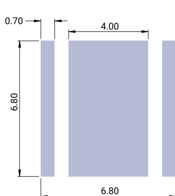
Recommended 6-V PCB Footprint (Thermal pad is electrically isolated)
