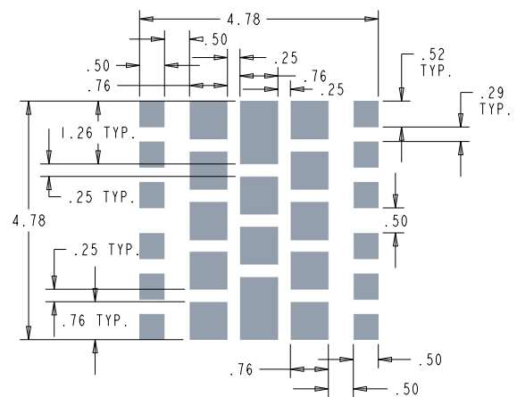
Recommended Solder Pad (Solder Mask Pattern)
