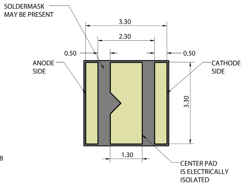
Bottom View
