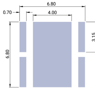
Recommended 6-V PCB Footprint Configuration Depending on Vf Class
