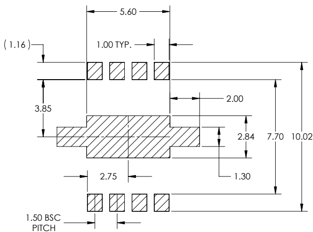
Recommended PCB Solder Pad
