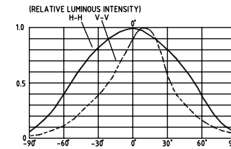
FIG.6a RED &amp; BLUE&amp;GREEN FAR FIELD PATTERN
