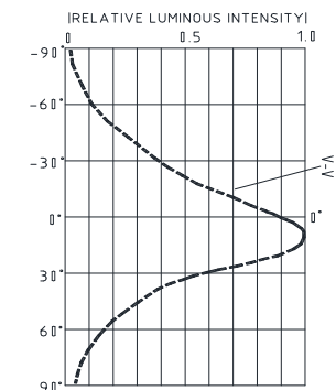
FIG.7 RED &amp; BLUE&amp;GREEN FAR FIELD PATTERN
