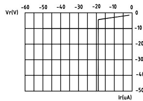
FIG.3b BLUE &amp; GREEN REVERSE CURRENT VS. REVERSE VOLTAGE.
