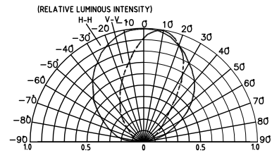
FIG.6b RED &amp; BLUE&amp;GREEN FAR FIELD PATTERN
