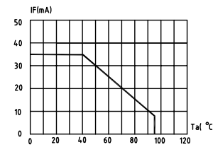
FIG.4b BLUE &amp; GREEN MAXIMUM FORWARD DC CURRENT VS. AMBIENT TEMPERATURE (Tjmax=105 °C)
