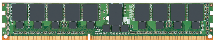
NVDIMM (24mm)
