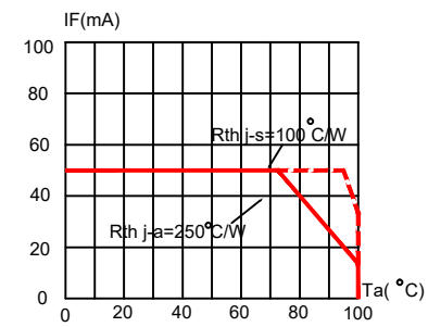
FIG.4 MAXIMUM FORWARD DC CURRENT VS AMBIENT TEMPERATURE ( T_{jmax}=110^{\circ}\text{C} )
