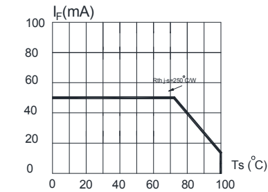
FIG.3 MAXIMUM FORWARD DC CURRENT VS SOLDER TEMPERATURE ( T_{jmax}=110^{\circ}C )
