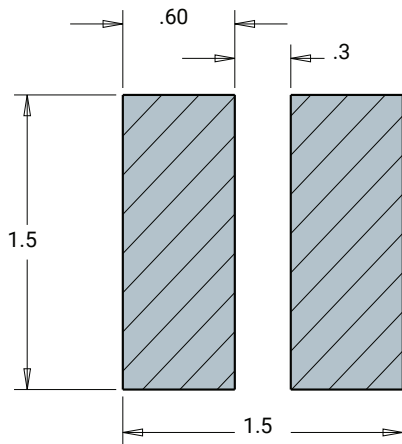
Recommended PC Board Solder Pad
