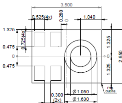
Stencil Pattern
