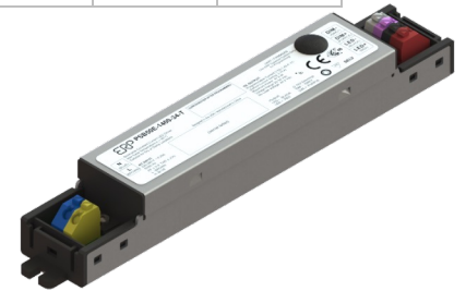
Terminal Blocks: "-T" Suffix L 154.2 x W 26.2 x H 21.85 mm (L 6.07 x W 1.03 x H 0.86 in.)
