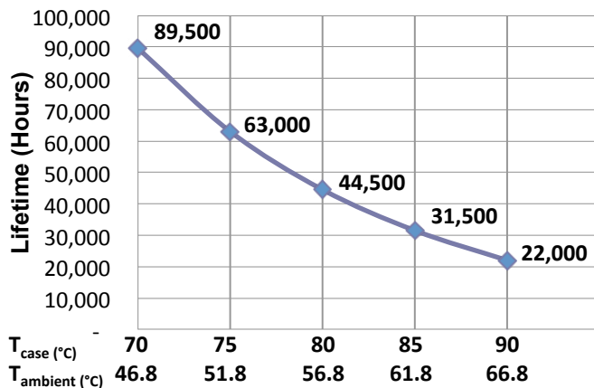
EVM080W-1750-42 (73.5 W, 1.75 A @ 42 V max) Predicted Lifetime versus Temperature
