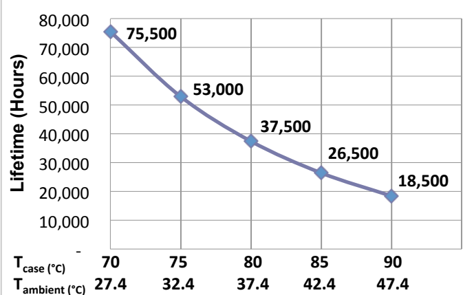
EVM120W-3000-40 (120 W, 3 A @ 40 V max) Predicted Lifetime versus Temperature
