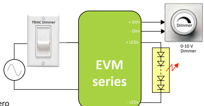
APPLICATION DIAGRAM
