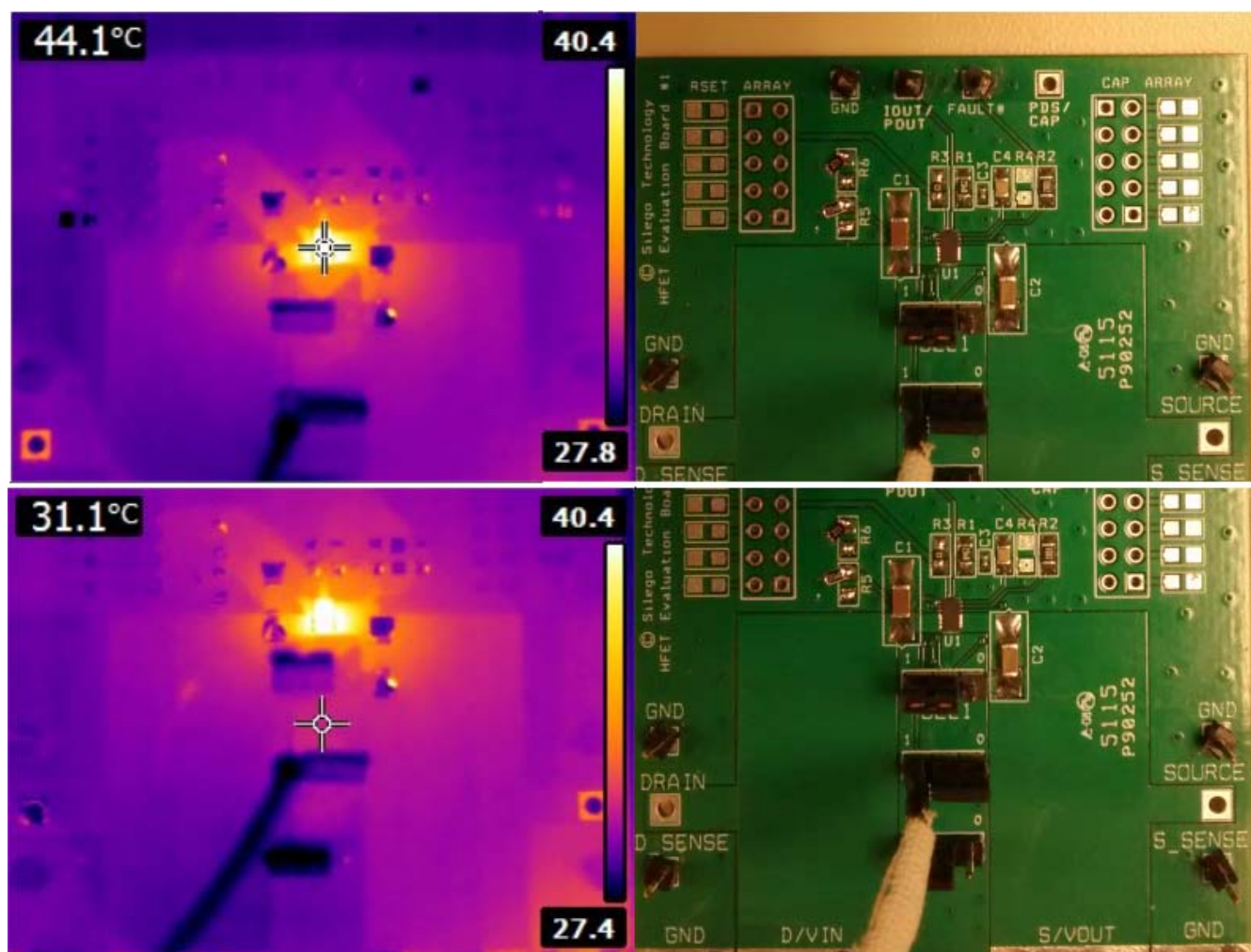
Figure 4. Thermal distribution for V_{IN} = 20 V, I_{DS} = 4.5 A after 2 min power up
