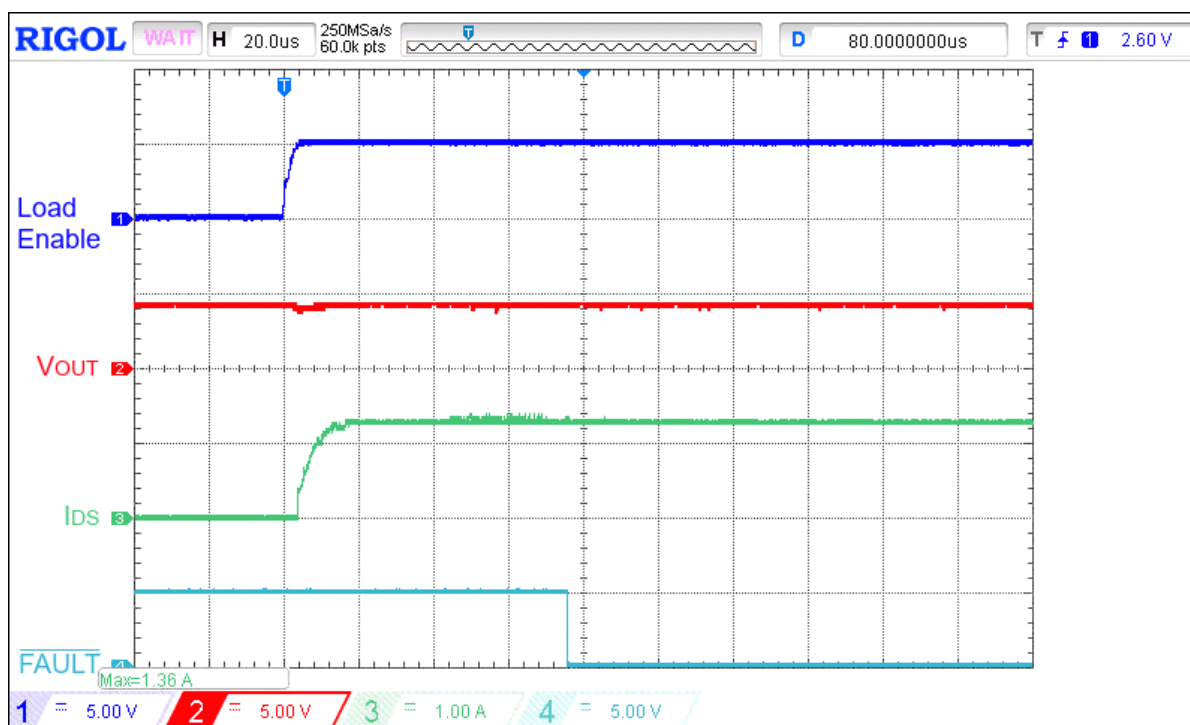
Figure 13. Typical FAULT assertion waveform for V_{IN} = 4.5 V, C_{LOAD} = 10 μF, I_{ACL} = 1 A, R_{SET} = 91 kΩ, switch on 3.3 Ω load
