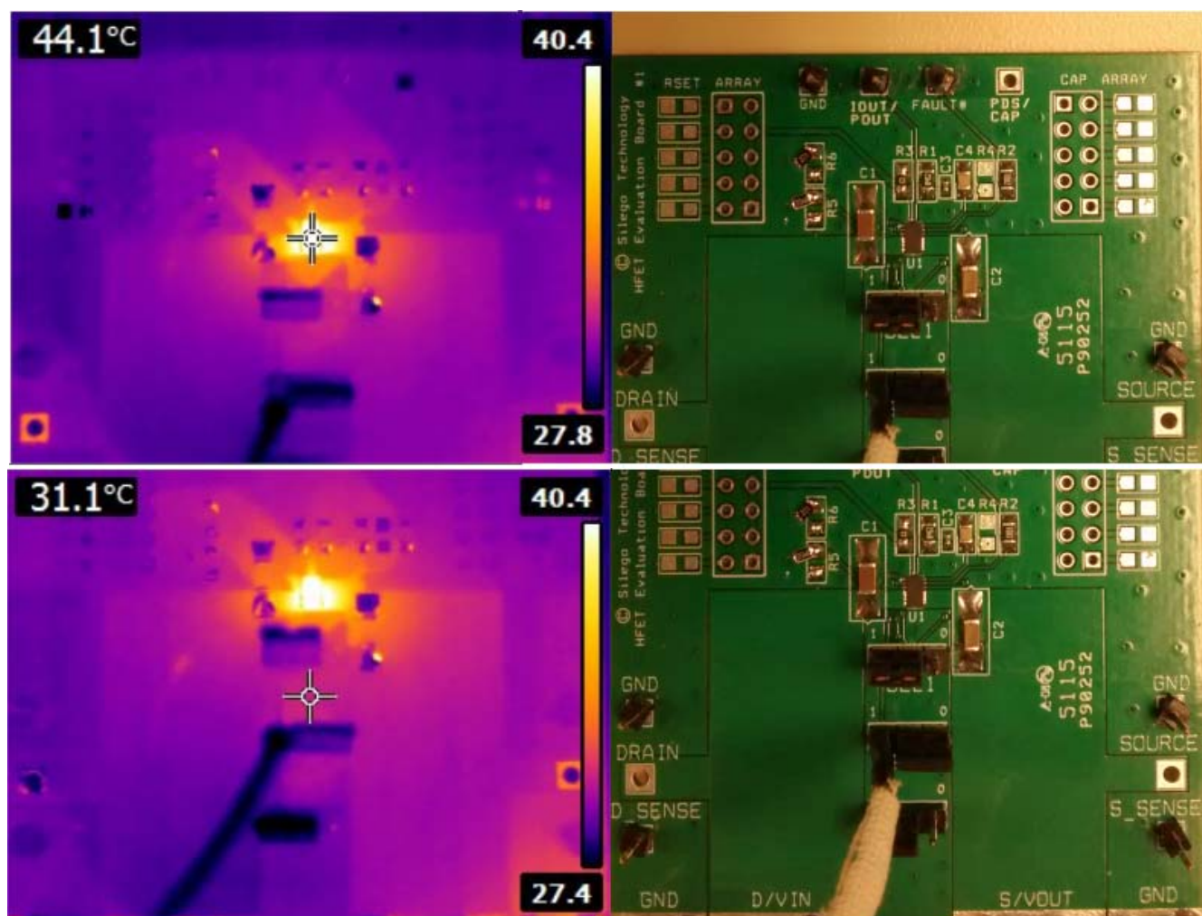
Figure 20. Thermal distribution for V_{IN} = 20 V, I_{DS} = 4.5 A after 2 min power up
