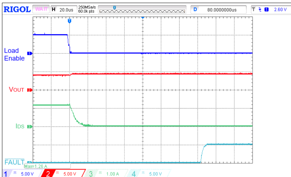
Figure 14. Typical FAULT de-assertion waveform for V_{IN} = 4.5 V, C_{LOAD} = 10 μF, I_{ACL} = 1 A, R_{SET} = 91 kΩ, switch out 3.3 Ω load
