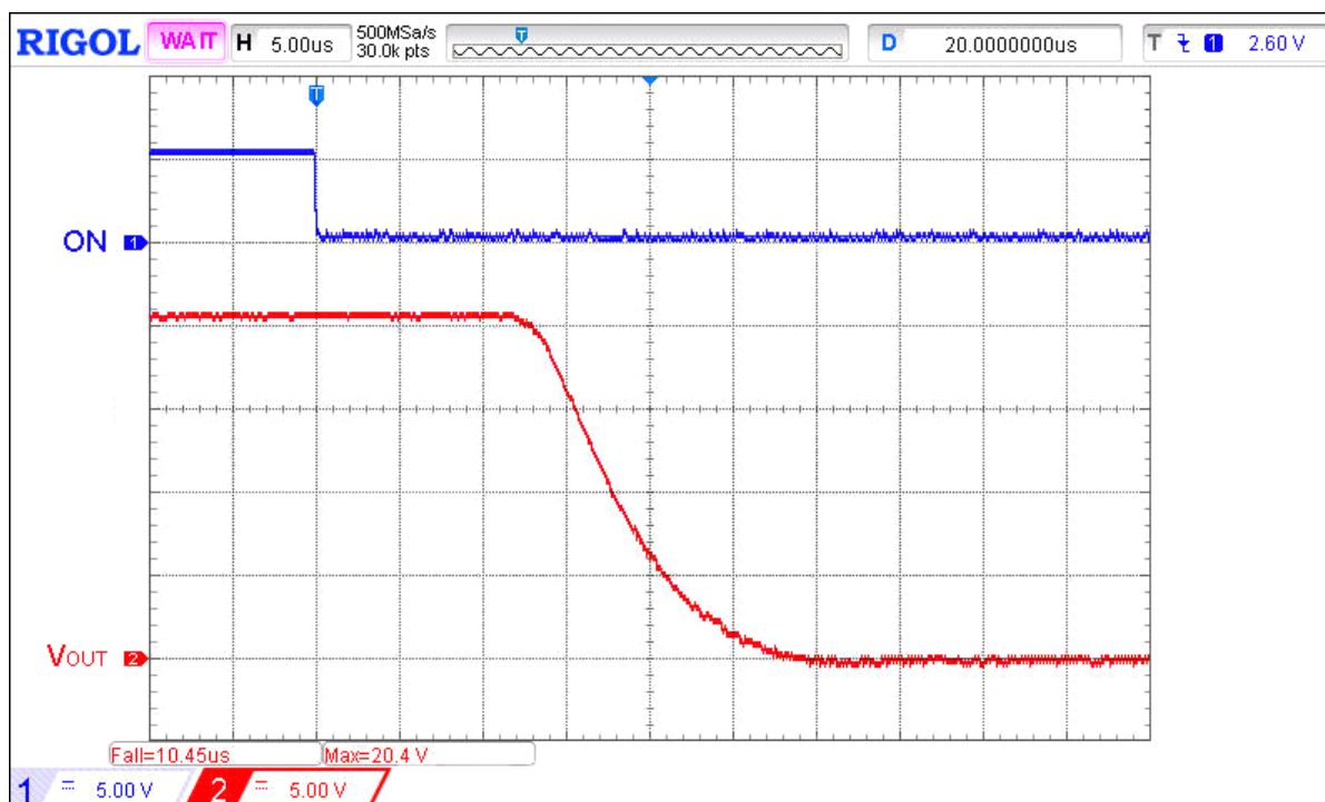
Figure 8. Typical Turn OFF operation waveform for V_{IN} = 20 V, C_{SLEW} = 10 nF, no C_{LOAD} , R_{LOAD} = 100 \Omega
