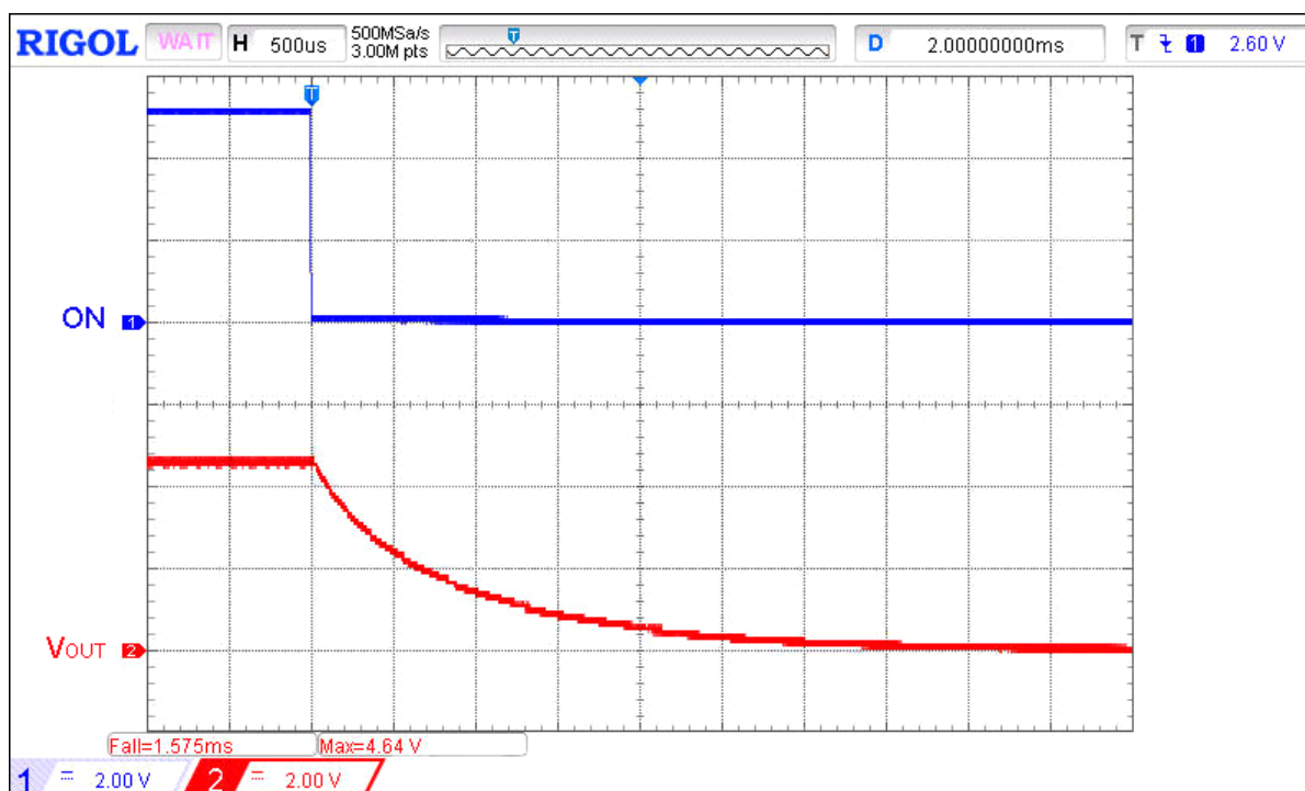
Figure 7. Typical Turn OFF operation waveform for V_{IN} = 4.5 V, C_{SLEW} = 10 nF, C_{LOAD} = 10 \mu F, R_{LOAD} = 100 \Omega
