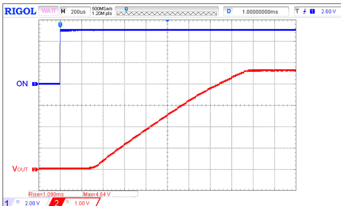
Figure 2. Typical Turn ON operation waveform for V_{IN} = 4.5 V, C_{SLEW} = 10 nF, C_{LOAD} = 10 μF, R_{LOAD} = 100 Ω
