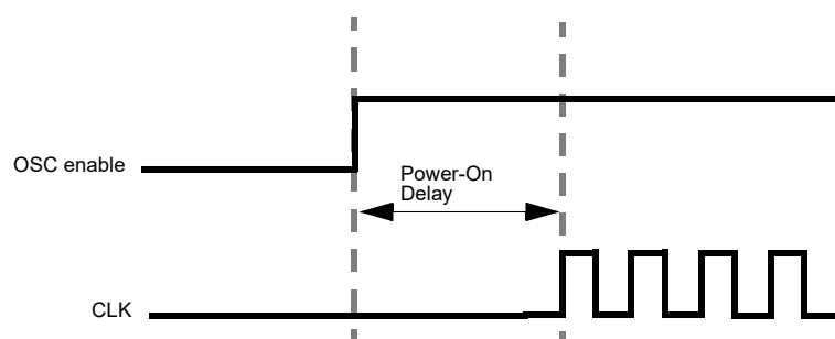
Figure 95: Oscillator Startup Diagram
