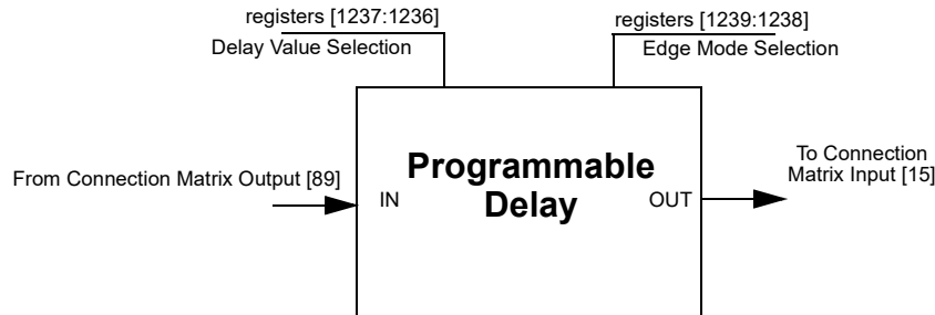
Figure 86: Programmable Delay
