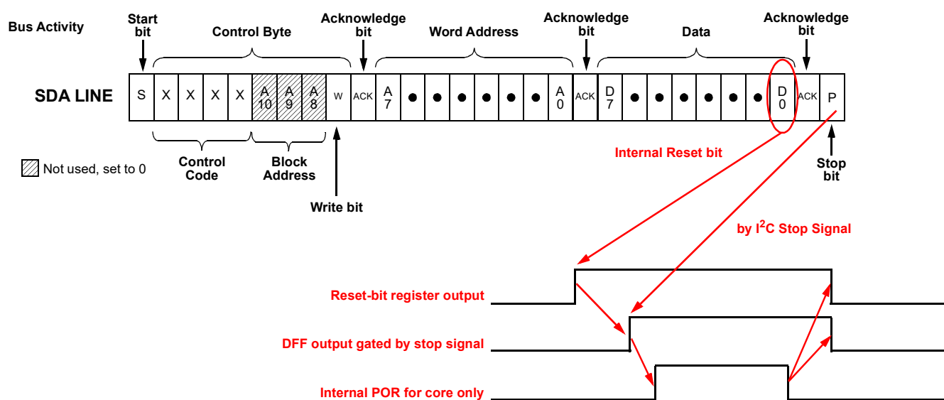
Figure 106: Reset Command Timing
