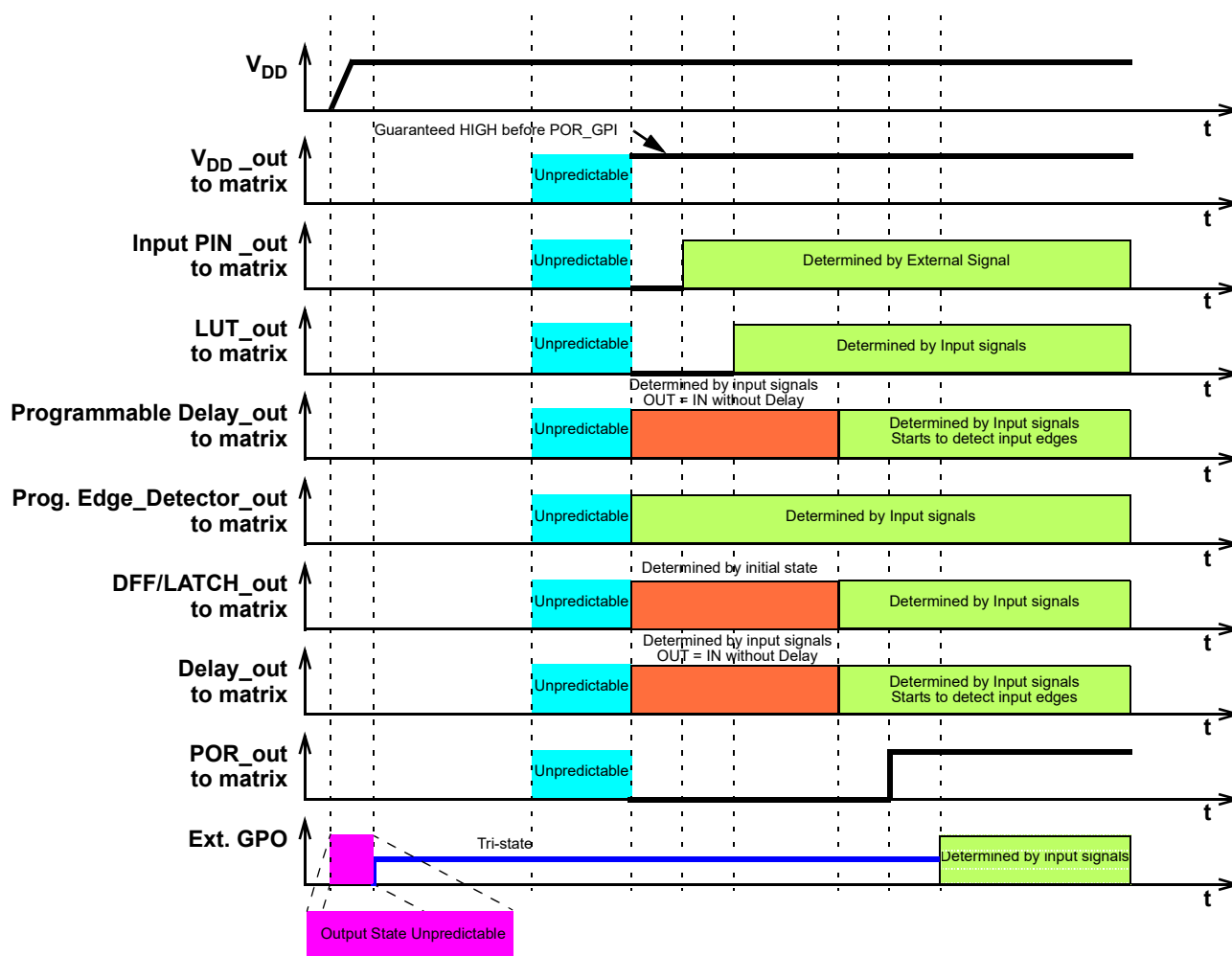
Figure 97: Internal Macrocell States During POR Sequence
