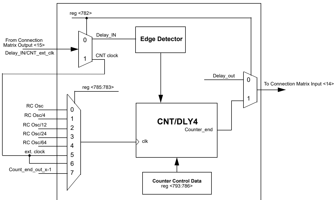
Figure 22. CNT/DLY4
