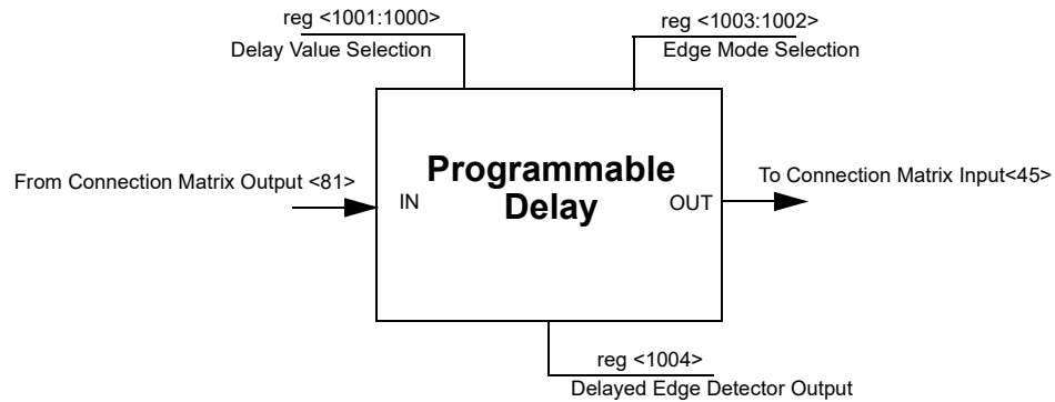
Figure 28. Programmable Delay
