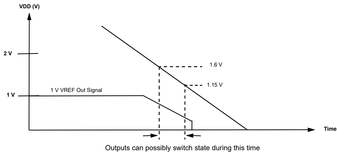
Figure 42. Power Down
