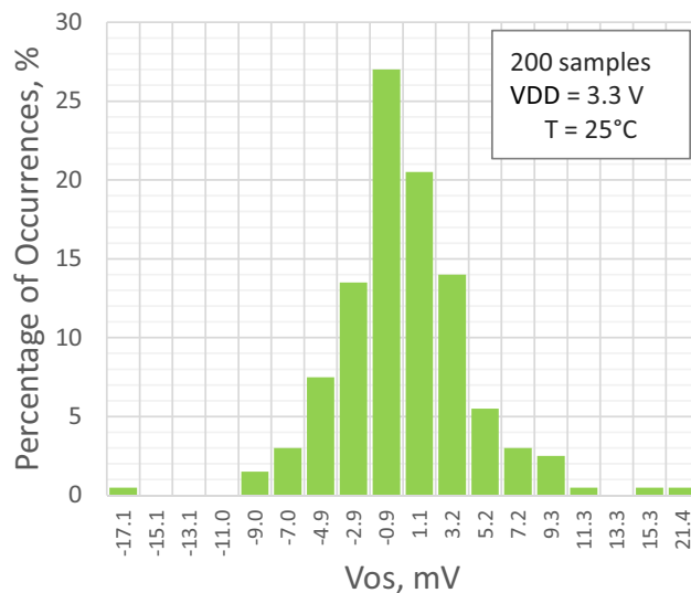
Figure 16. PGA Input Offset Distribution, Single-Ended Mode, G = 0.5
