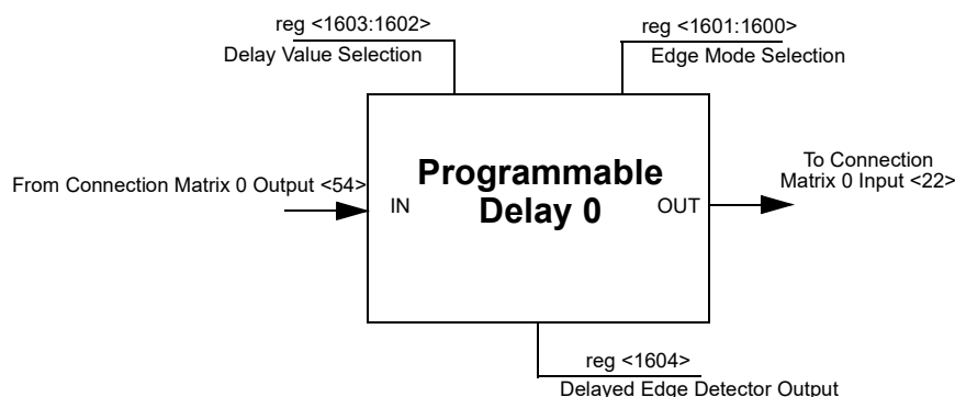
Figure 108. Programmable Delay
