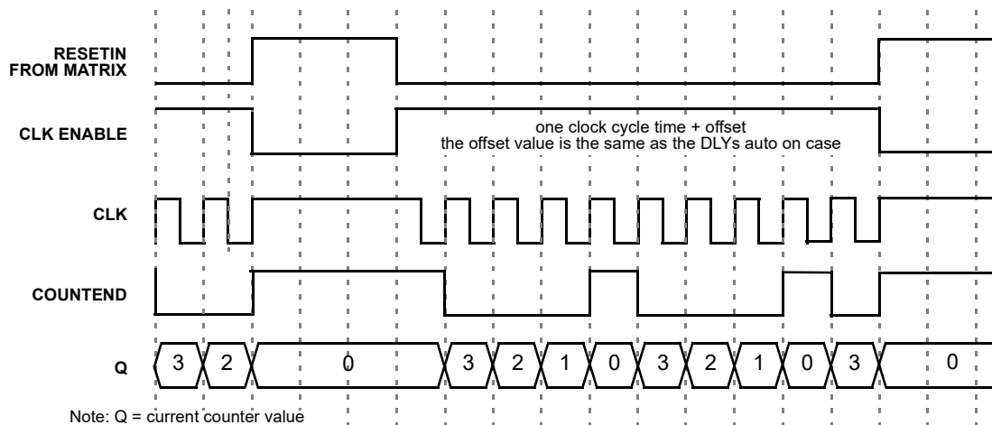
Figure 91. Timing (reset high level mode, oscillator is autpowered on (controlled by reset)) for count data = 3
