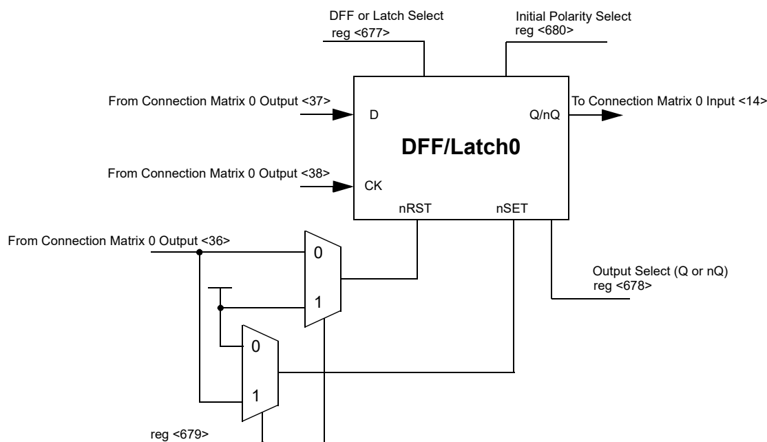
Figure 62. DFF/Latch0
