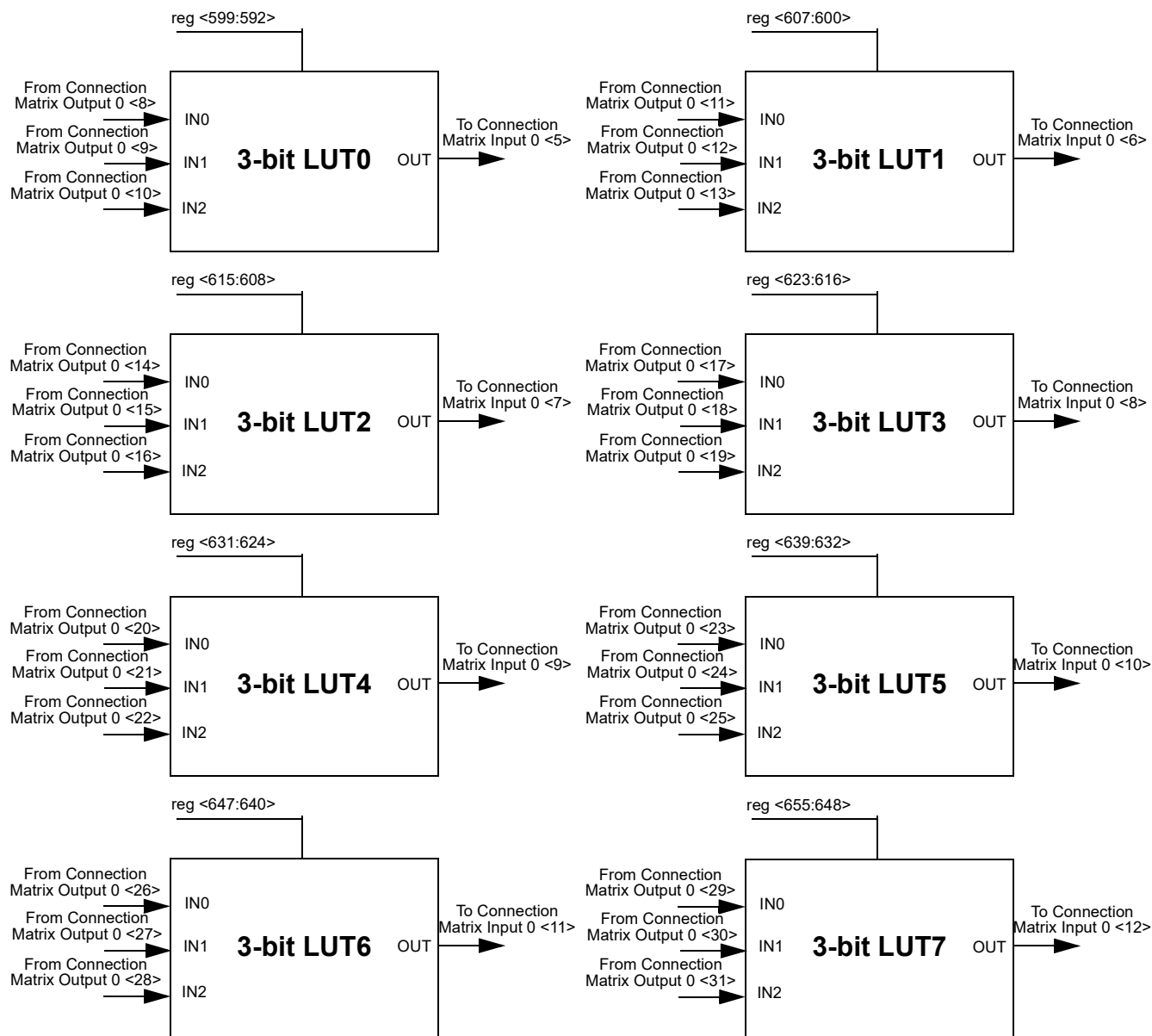
Figure 43. 3-bit LUTs
