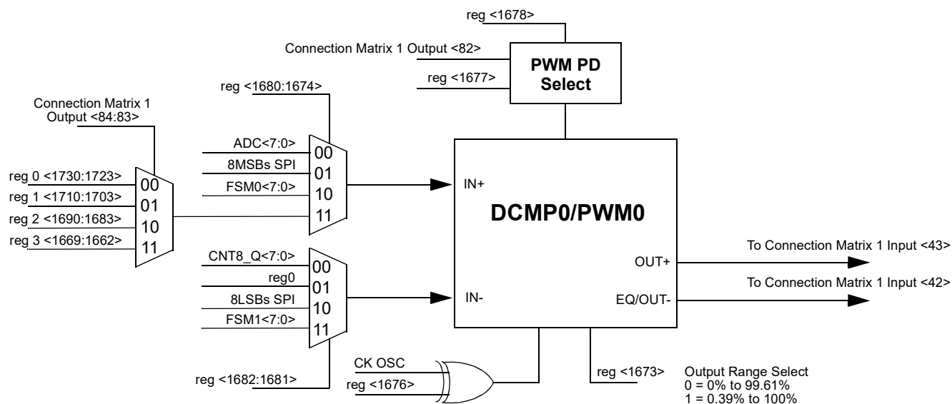
Figure 97. DCMP0/PWM0 Functional Diagram
