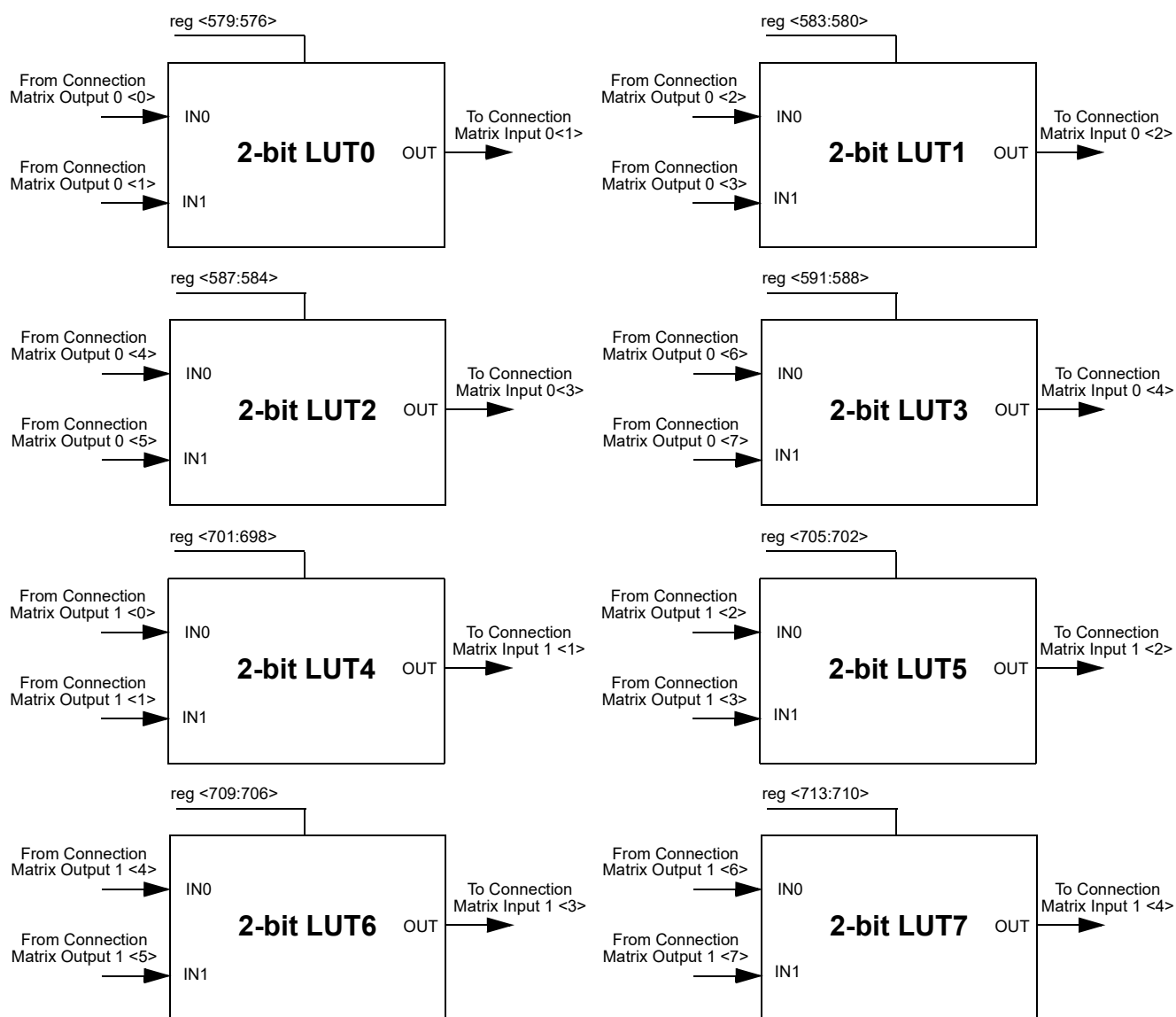
Figure 42. 2-bit LUTs
