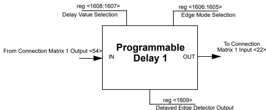
Figure 109. Programmable Delay
