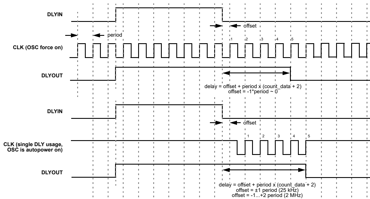
Figure 88. Timing (falling edge) for count data = 3
