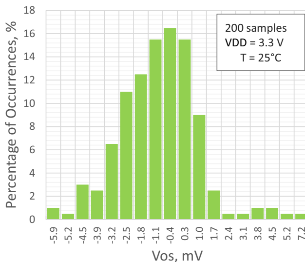
Figure 18. PGA Input Offset Distribution, Single-Ended Mode, G = 2
