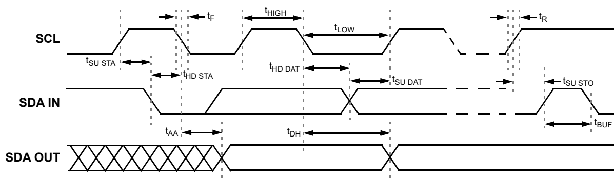
Figure 102. I 2 C General Timing Characteristics
