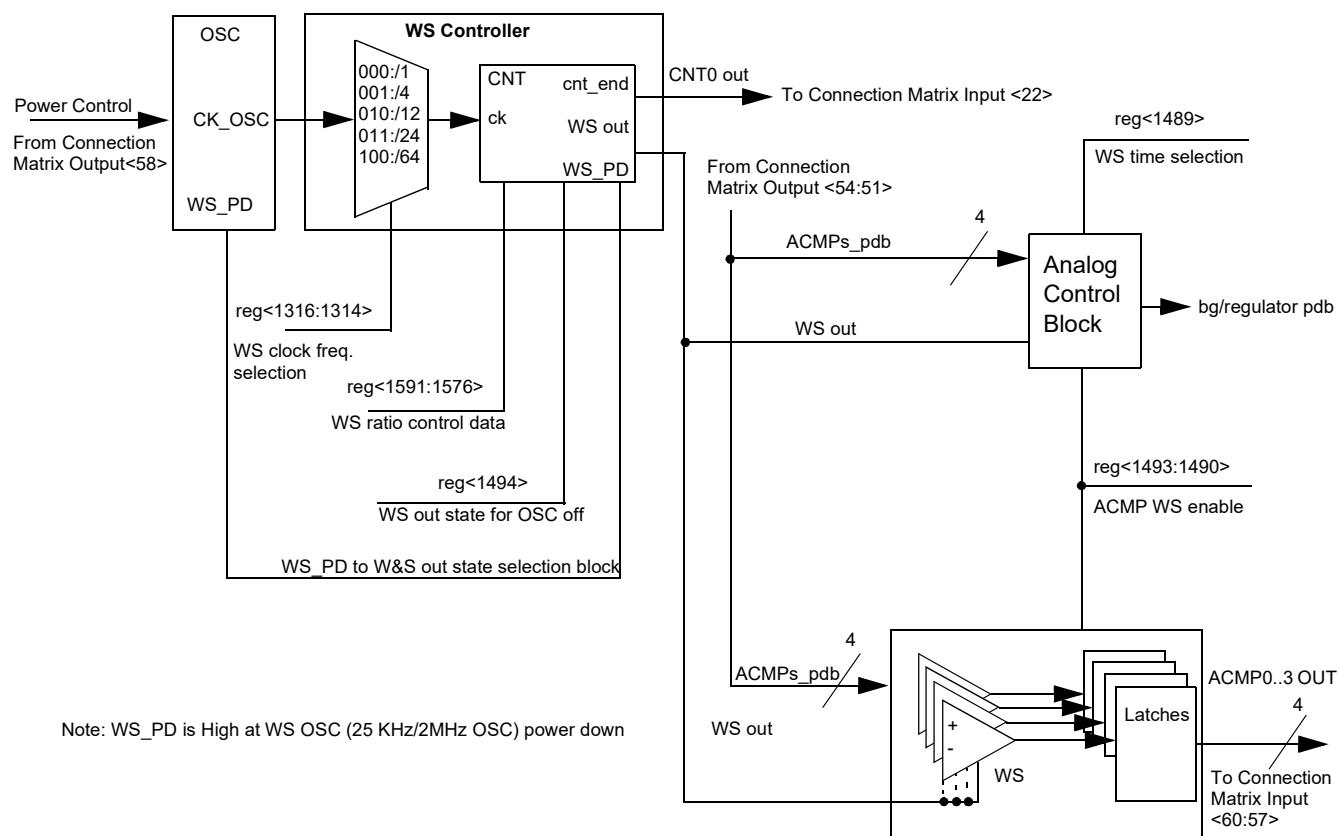
Figure 49. WS controller
