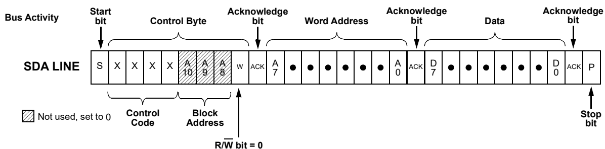
Figure 78. Byte Write Command, \overline{R/\overline{W}} = 0
