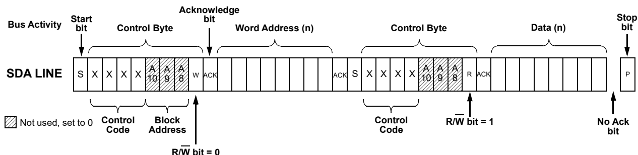
Figure 81. Random Read Command
