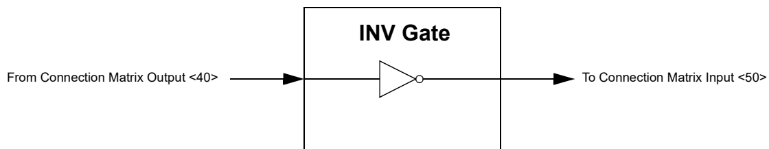
Figure 62. INV Gate
