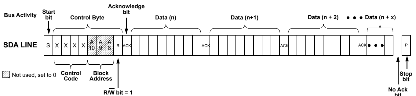
Figure 101. Sequential Read Command
