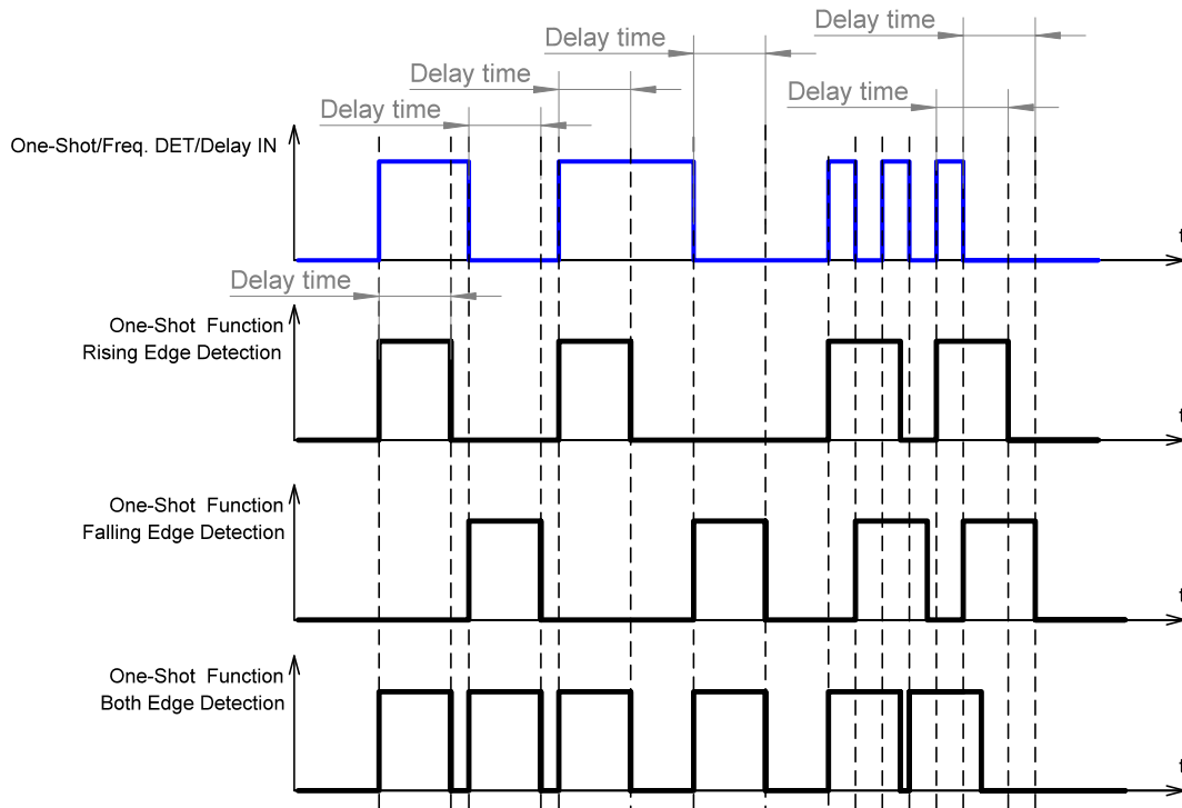
Figure 31. One-shot function
