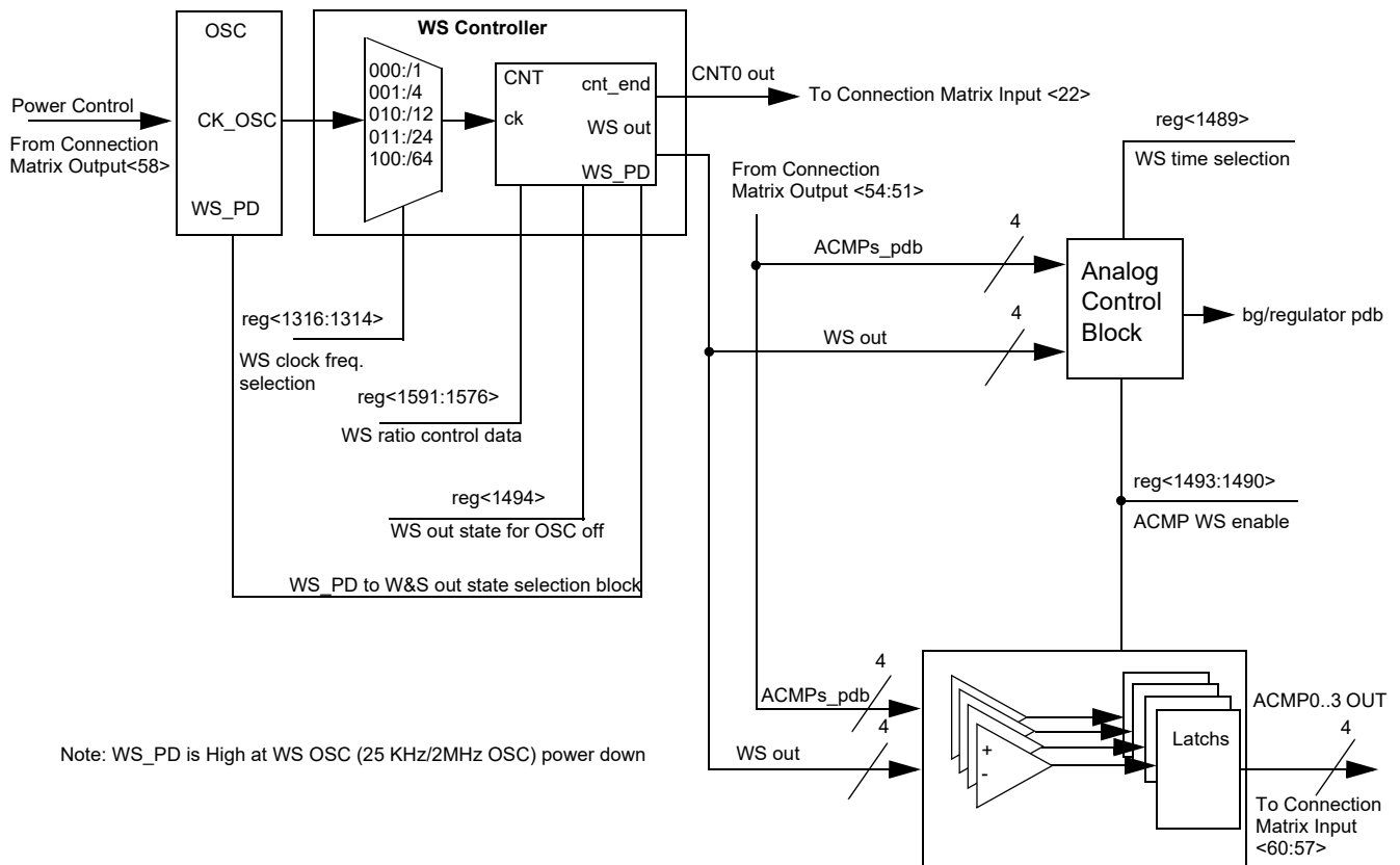
Figure 37. WS controller
