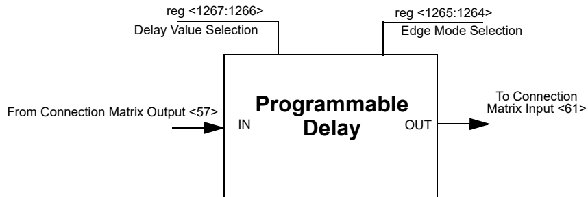
Figure 47. Programmable Delay
