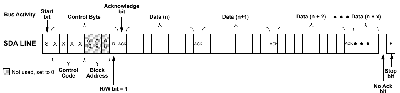
Figure 91. Sequential Read Command
