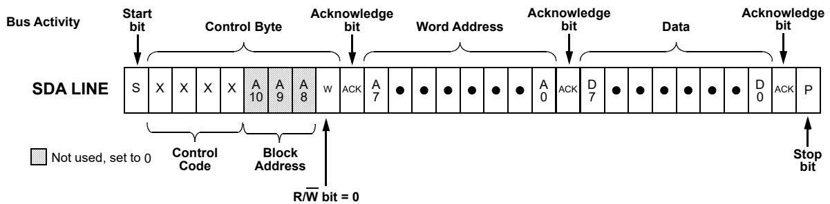
Figure 87. Byte Write Command, \overline{R/\overline{W}} = 0
