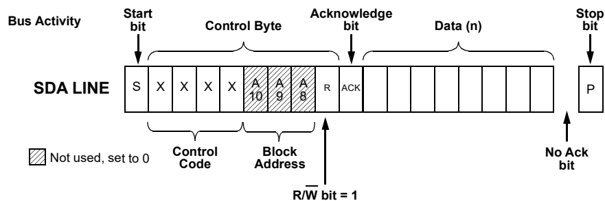
Figure 87. Current Address Read Command, \overline{R/W} = 1
