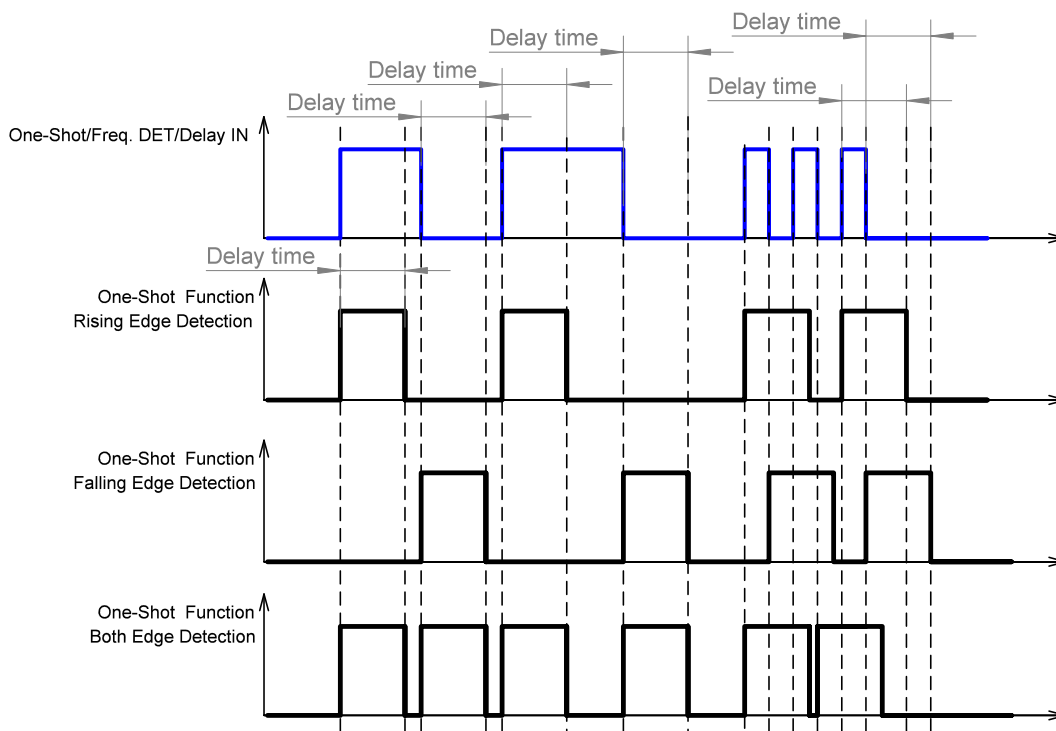
Figure 30. One-shot function
