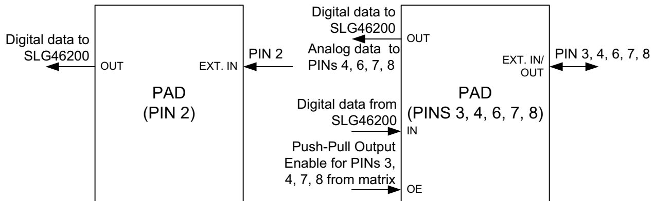
Figure 2. I/O Pads Layout
