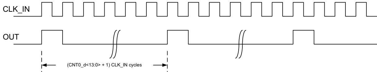
Figure 23. Counter Behavior
