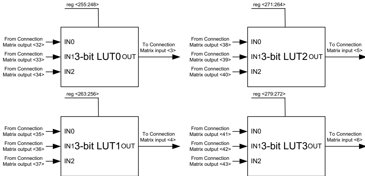
Figure 31. 3-bit LUTs
