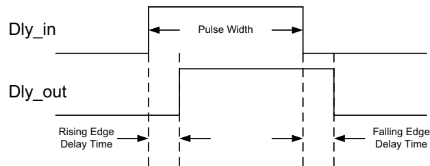
Figure 28. Delay Cells - Rising and Falling Edge
