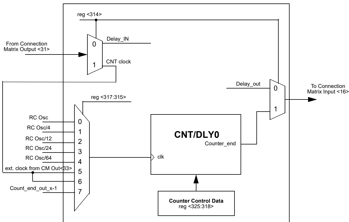
Figure 36. CNT/DLY0
