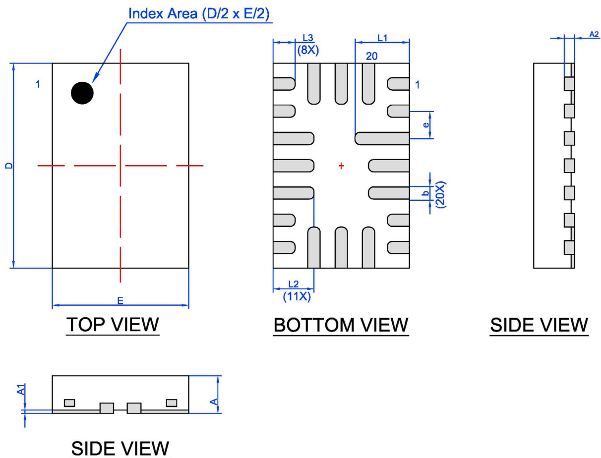
20 Lead STQFN Package JEDEC MO-220, Variation WECE
