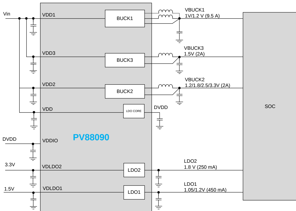
Figure 2: Block Diagram
