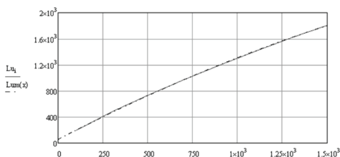
Figure 9.4 : Scaled Diode Curve
