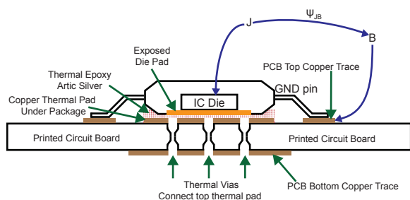
Figure 9.14 : Ways to Improve Thermal Resistance
