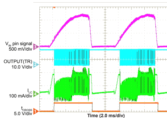
Figure 9.6 : Signals of Chopping Circuit.
