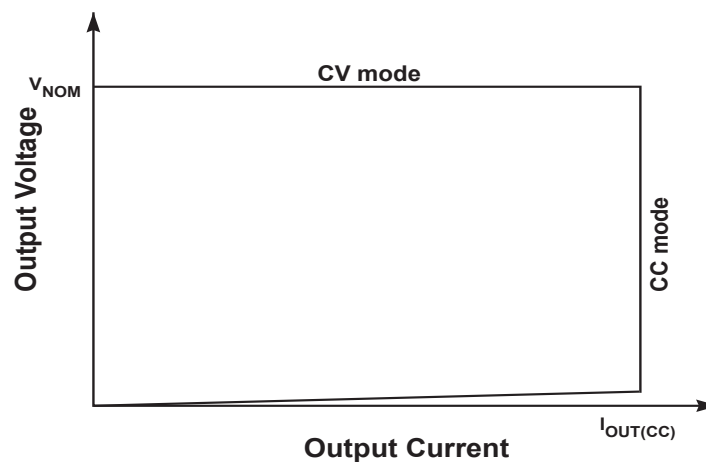
Figure 10.4 : Power Envelope
