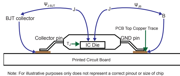
Figure 10.6 : Thermal Resistance
