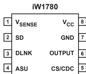
Pin Number Pin Name Type Pin Description 1 V SENSE Analog Input Auxiliary voltage sense. Used for primary-side regulation. 2 SD Analog Input External shutdown control. Can be configured for external over-temperature protection (OTP) by connecting an NTC resistor from this pin to Ground. 3 DLNK Analog Input Digital communication link signal. Used for secondary-side to primary-side communication for all rapid charge information, which includes output voltage requests, output current limits, output voltage undershoot, and over-voltage protection. 4 ASU Output Control signal. Used for active start-up device (BJT or depletion mode N-FET). 5 CS/CDC Analog Input Primary-side current sense and external cable drop compensation (CDC). Used for cycle-by-cycle peak-current control and limit in primary-side CV/CC regulation. Also used for CDC configuration. 6 OUTPUT Output Gate drive for external MOSFET switch. 7 GND Ground Ground. 8 V CC Power Input IC power supply.
