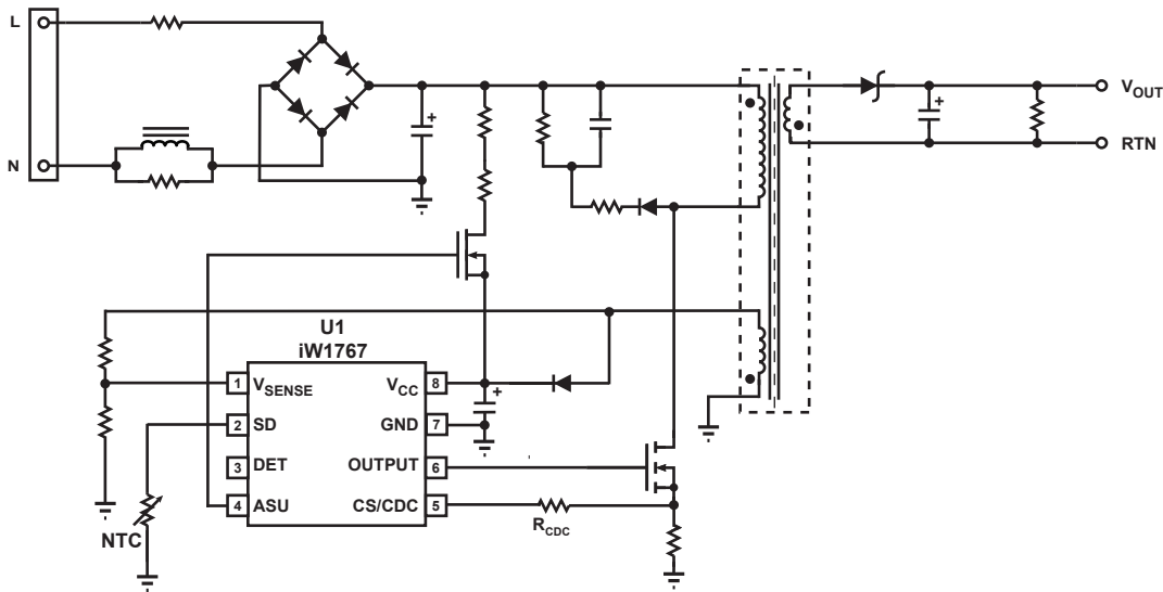
Figure 3.2: iW1767 Typical Application Circuit (Using Depletion Mode N-FET as Active Start-up Device)
