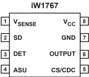
Figure 4.1: 8 Lead SO-8 Package
