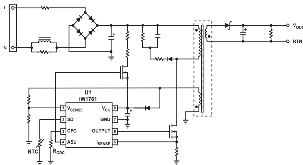
Figure 3.1: iW1761 Typical Application Circuit (Using Depletion Mode N-FET as Active Start-up Device) (Achieving < 10\text{mW} No-load Power Consumption in 5\text{V}/2\text{A} , 10\text{W} Adapter Designs)
