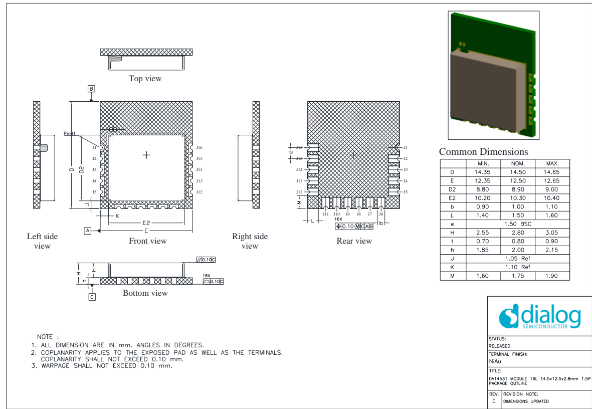
Figure 3: Mechanical Drawing
