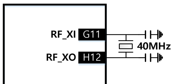
Figure 10: DA16200 3.8 × 3.8fcCSP Crystal Clock Connections
