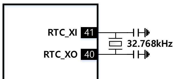
Figure 7: DA16200 6×6 QFN RTC Crystal Connections
