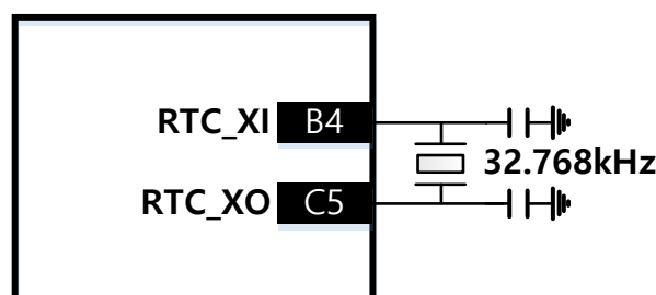
Figure 8: DA16200 3.8 × 3.8 fcCSP RTC Crystal Connections
