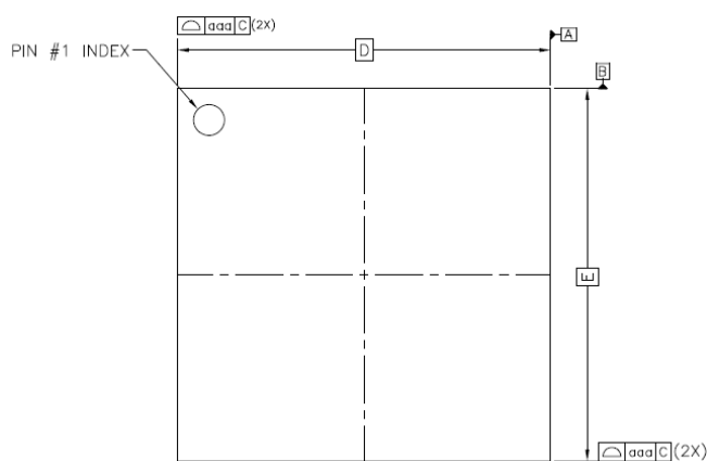
Figure 56: Top View
