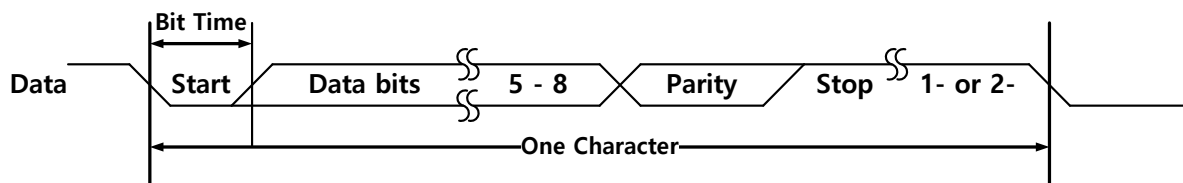
Figure 43: Serial Data Format
