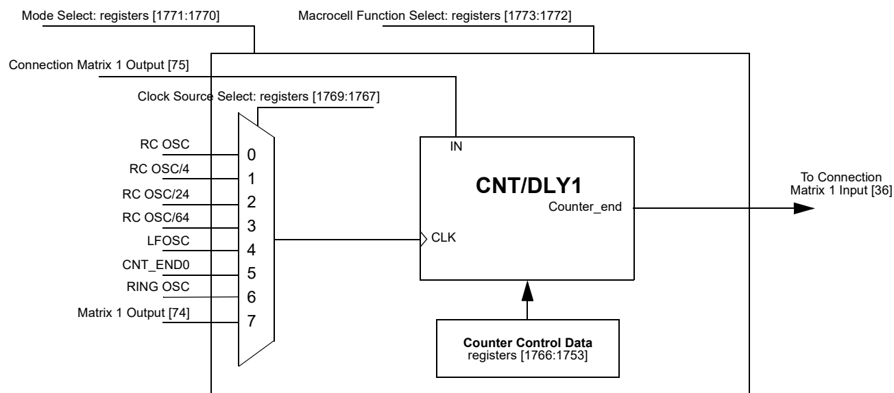
Figure 63: CNT/DLY1
