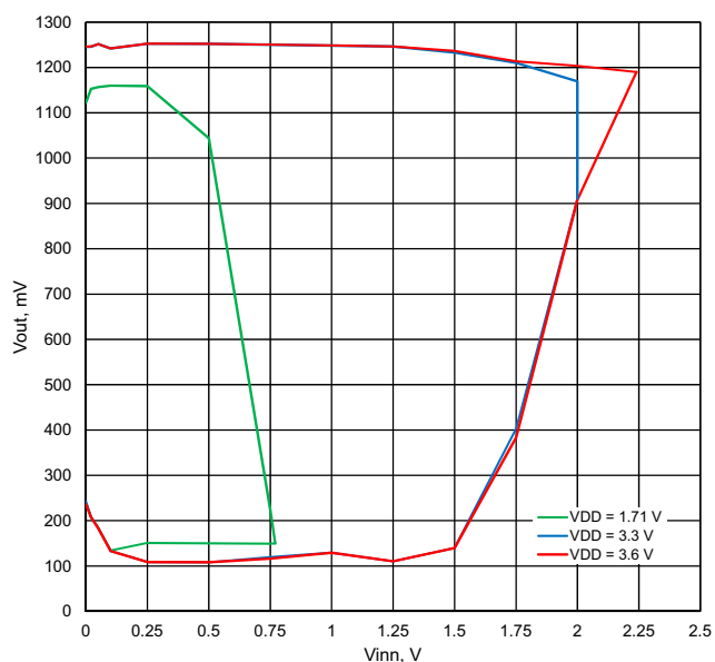
Figure 24: Typical Negative Input Voltage Range vs. Linear Output Voltage, Pseudo-Differential Mode, G = 2
