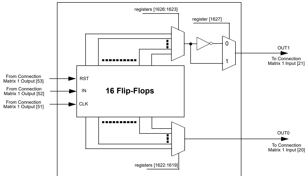
Figure 92: Pipe Delay 1
