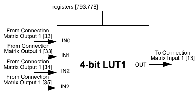
Figure 34: 4-bit LUT_1
