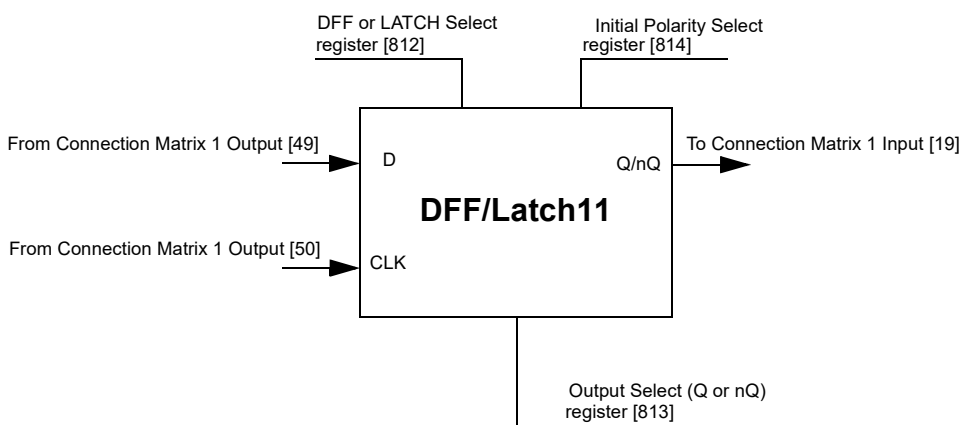
Figure 58: DFF/Latch11
