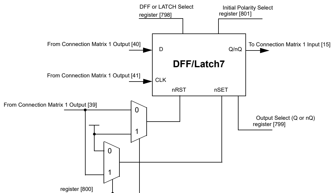
Figure 54: DFF/Latch7
