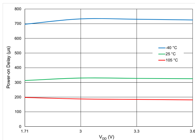
Figure 38: Maximum Power-On Delay vs. V_{DD} , BG = 100 \mu s, Regulator and Charge Pump set to automatic ON/OFF
