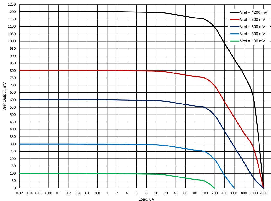
Figure 99: Typical Load Regulation, T = 25^{\circ}\text{C} , V_{\text{DD}} = 3.3 \text{ V}
