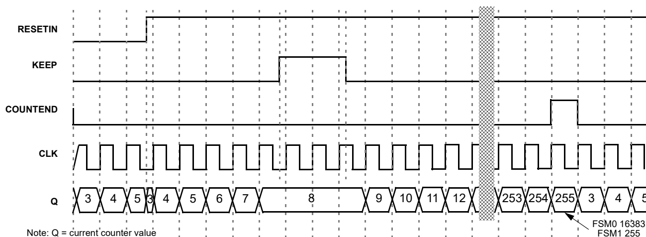
Figure 80: CNT/FSM Timing Diagram (Set Rising Edge Mode, Oscillator is Forced on, UP=1) for Counter Data = 3
