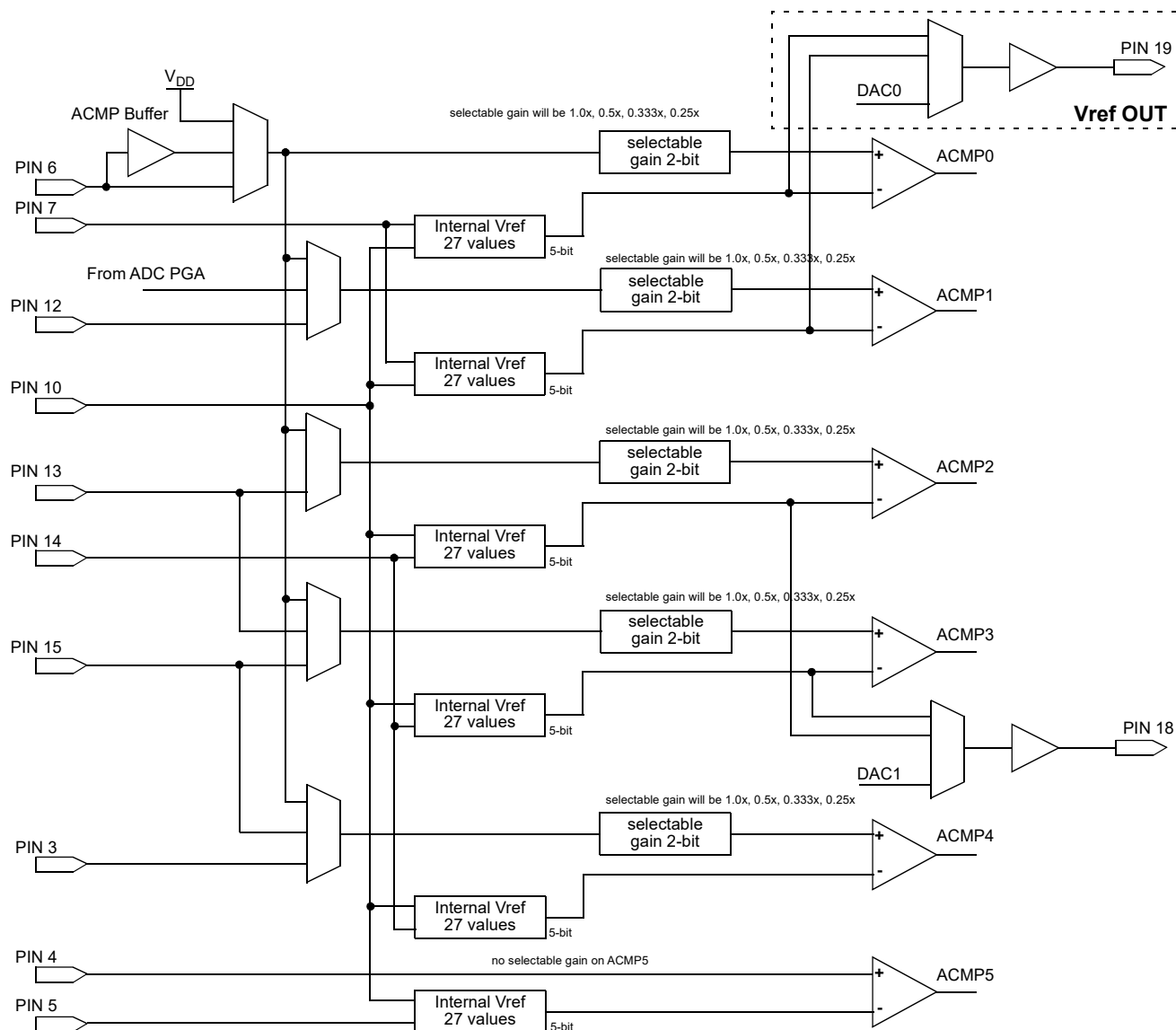
Figure 39: ACMP Master Architecture Diagram
