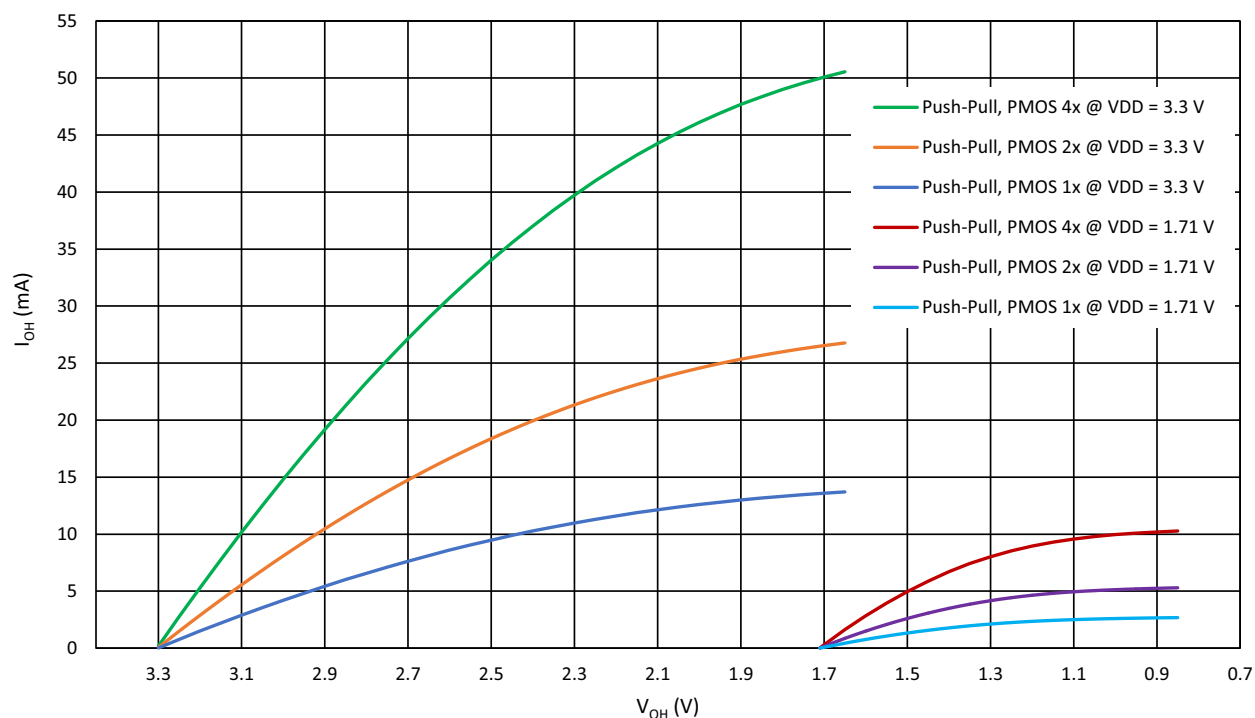
Figure 7: Typical High Level Output Current vs. High Level Output Voltage at T = 25^\circ\text{C}
