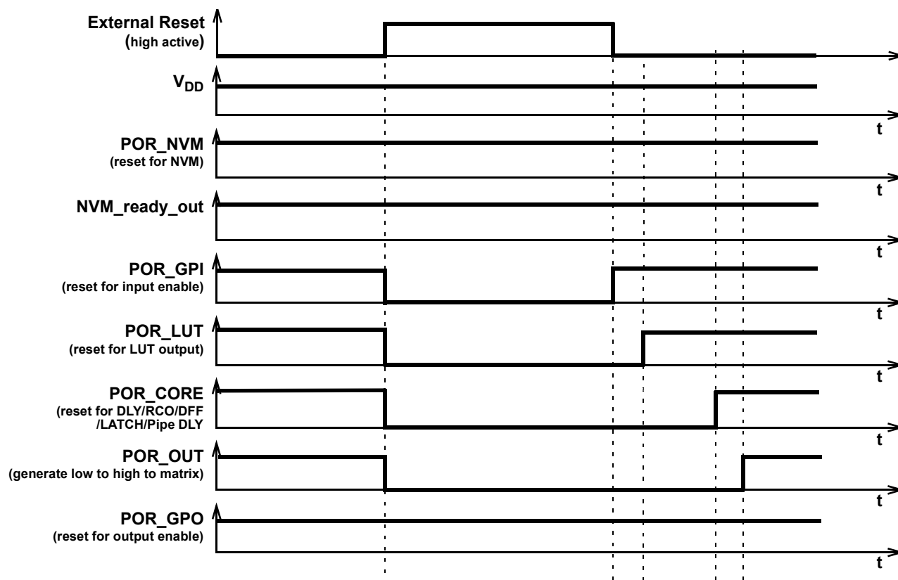
Figure 113: External Reset Sequence (High Active).
