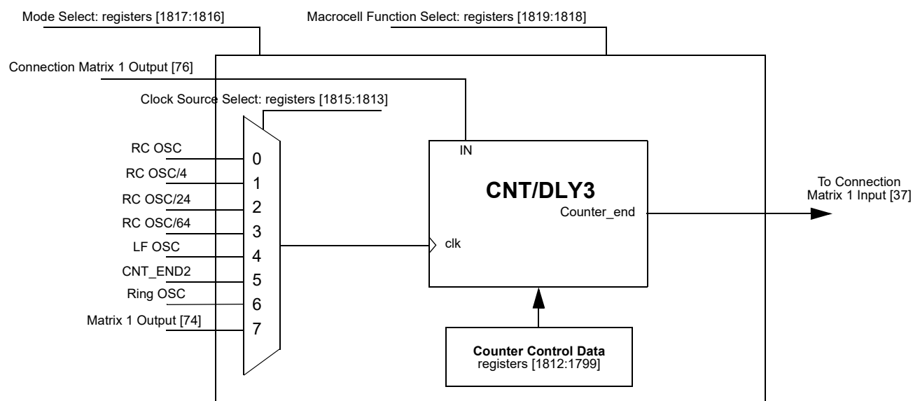
Figure 65: CNT/DLY3
