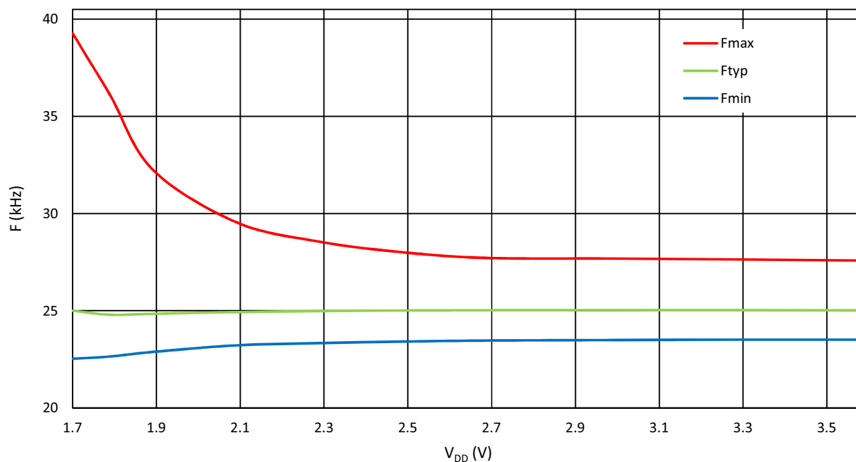
Figure 107: RC Oscillator Frequency vs. V_{DD} , RC OSC = 25 kHz, T = -40^{\circ}\text{C} to 105^{\circ}\text{C}
