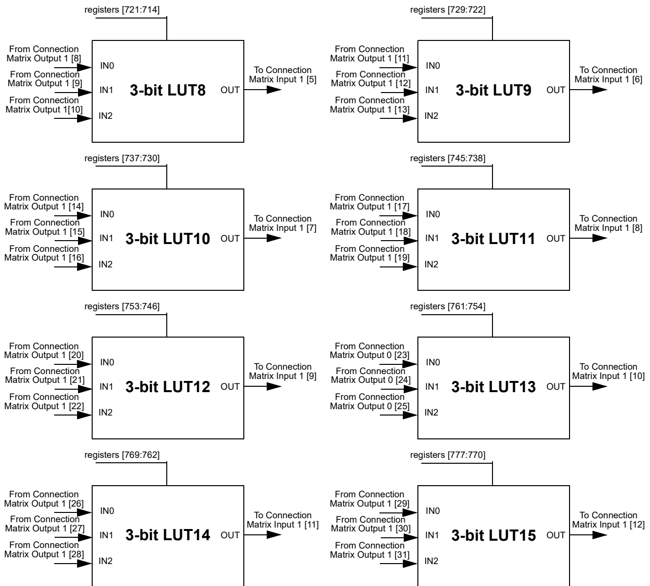
Figure 33: 3-bit LUTs
