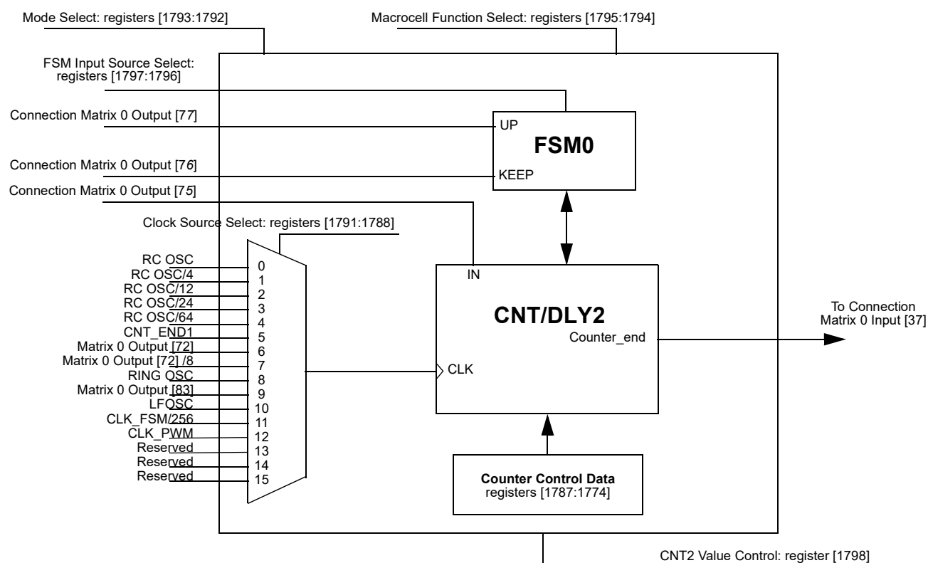
Figure 64: CNT/DLY2/FSM0
