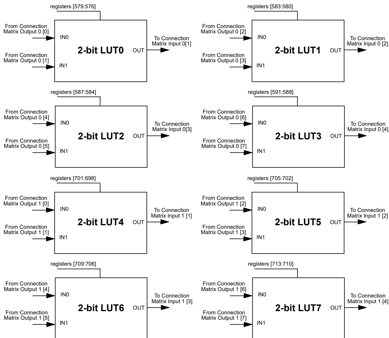
Figure 31: 2-bit LUTs
