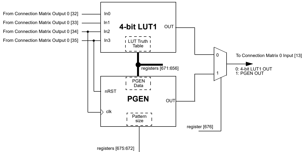
Figure 35: 4-bit LUT1 or PGEN
