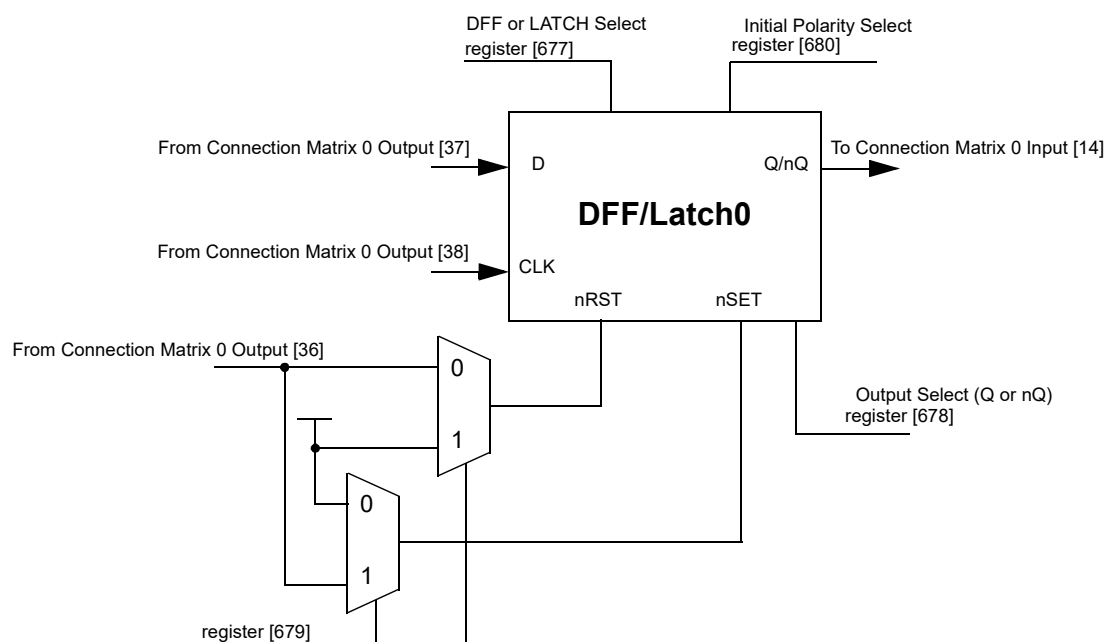
Figure 47: DFF/Latch0
