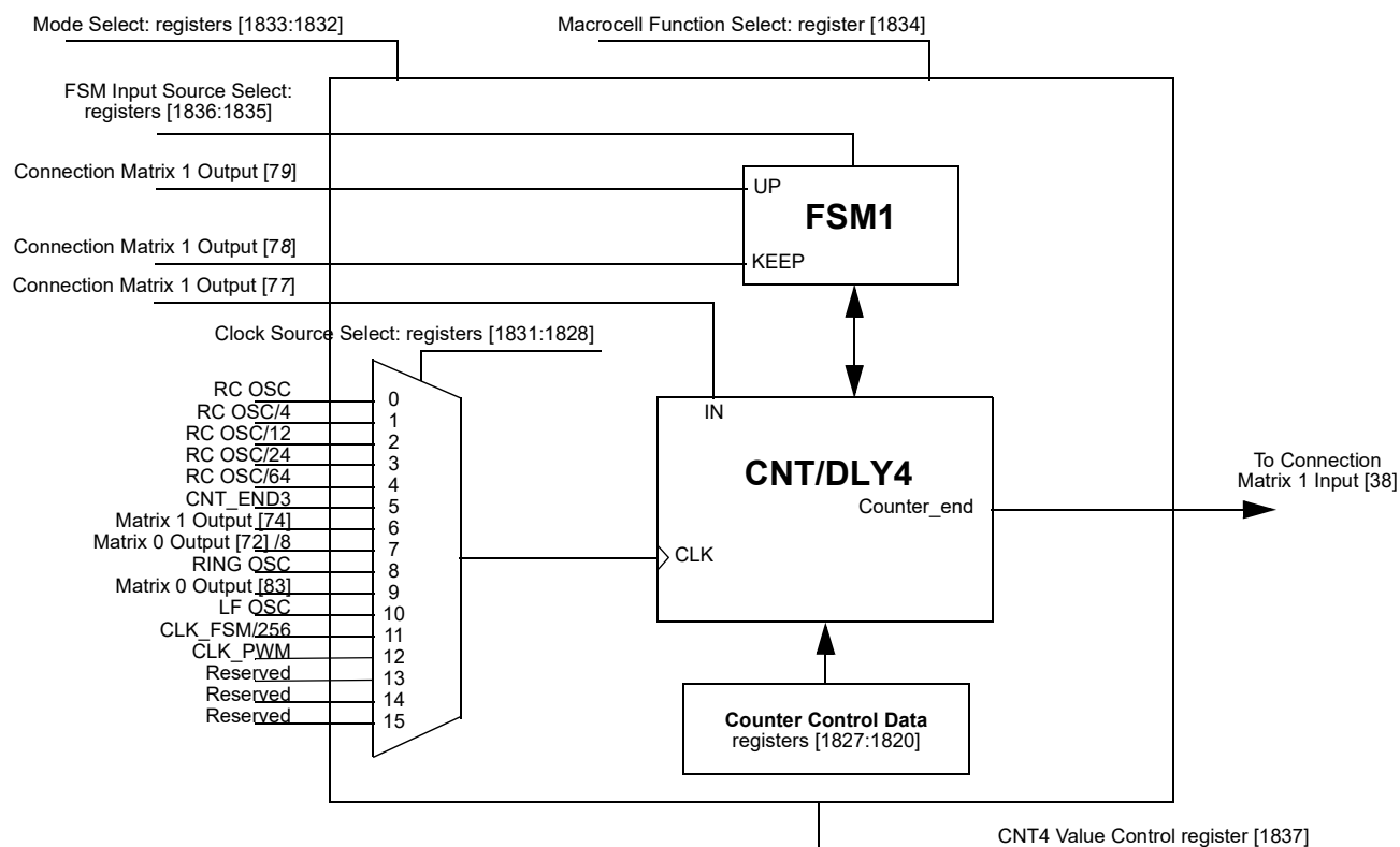
Figure 66: CNT/DLY4/FSM0
