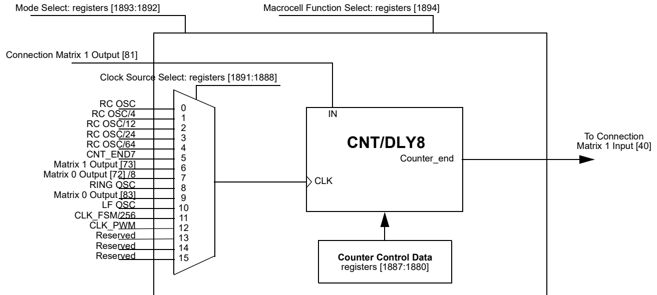
Figure 70: CNT/DLY8/PWM_RAMP
