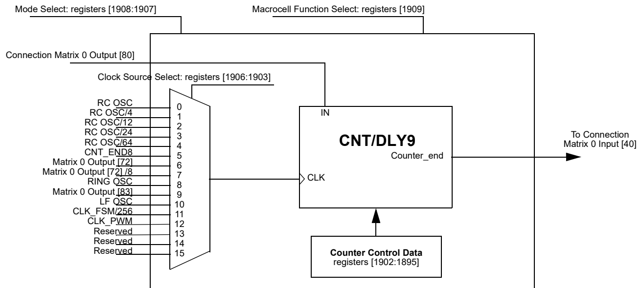
Figure 71: CNT/DLY9/PWM_RAMP
