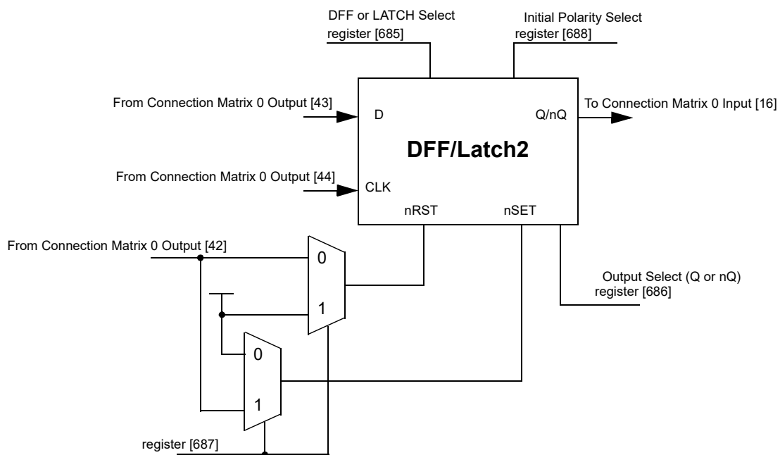
Figure 49: DFF/Latch2
