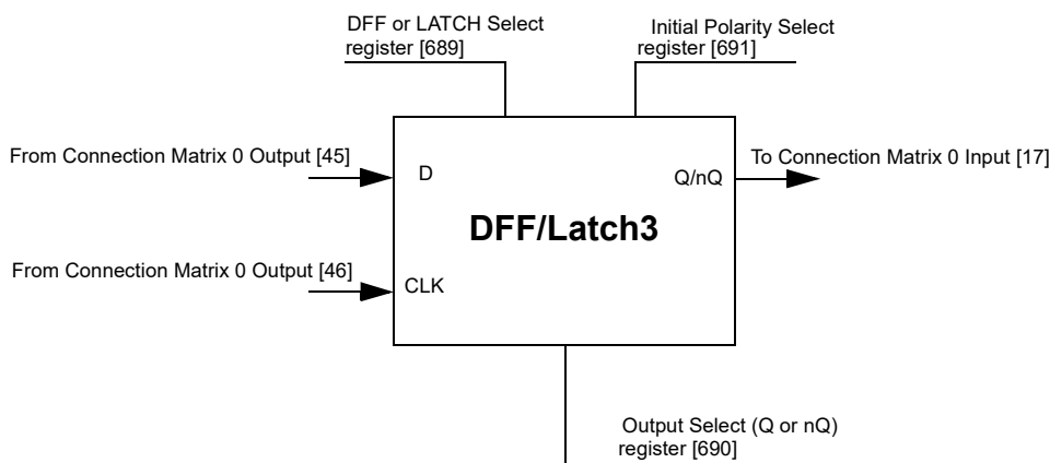
Figure 50: DFF/Latch3
