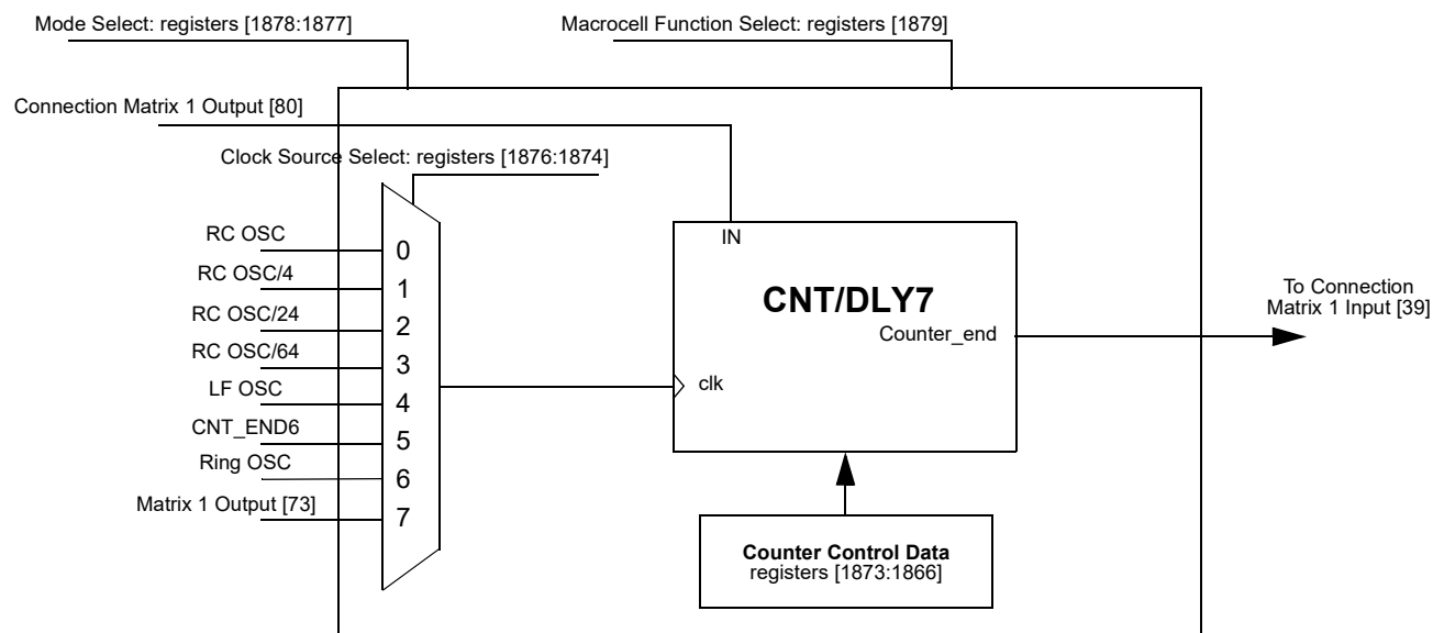
Figure 69: CNT/DLY7
