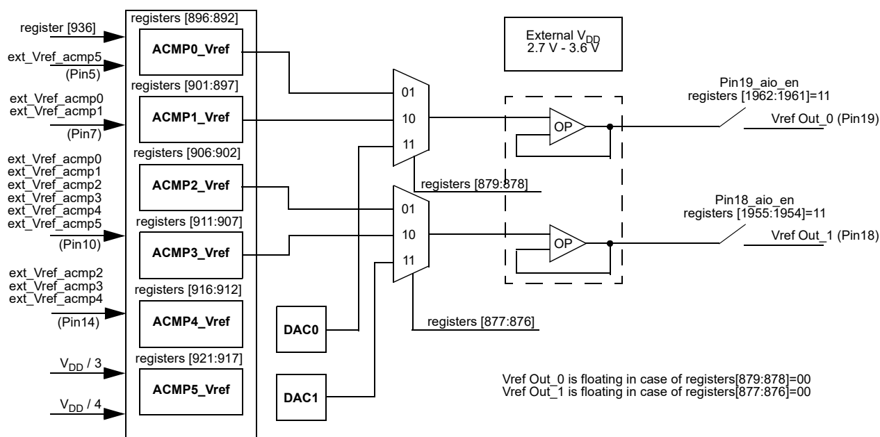
Figure 98: Voltage Reference Block Diagram
