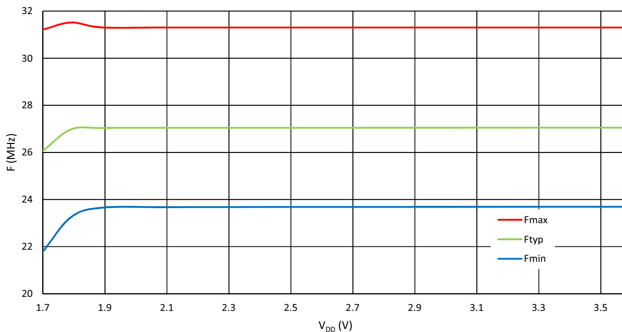
Figure 108: Ring Oscillator Frequency vs. V_{DD} , OSC = 27 MHz, T = 25^{\circ}\text{C}
