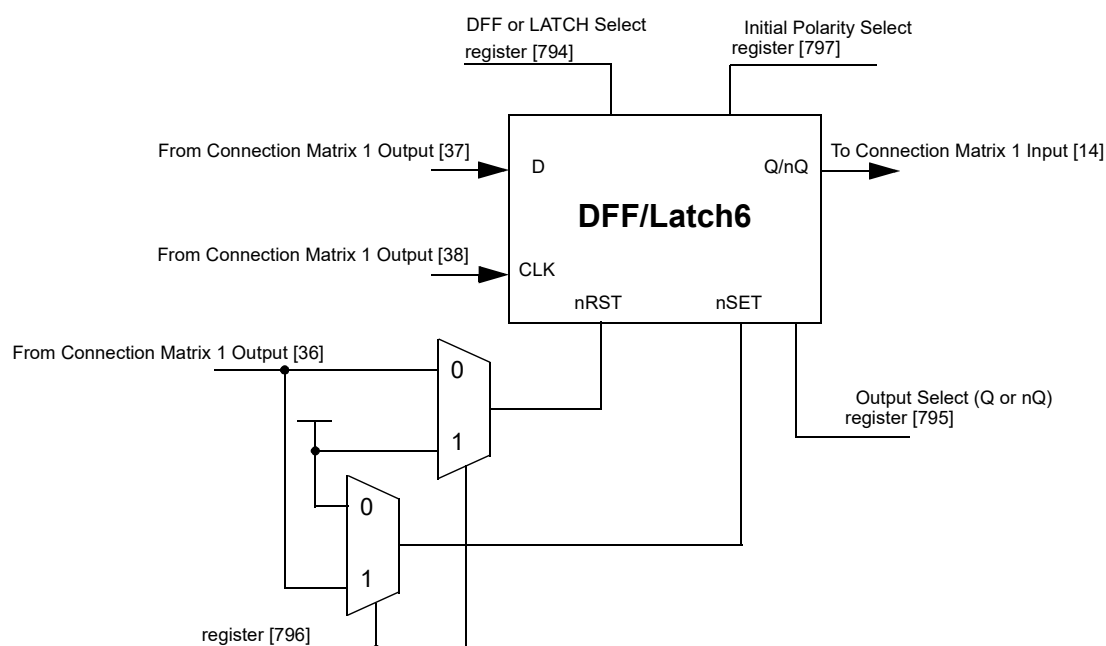
Figure 53: DFF/Latch6
