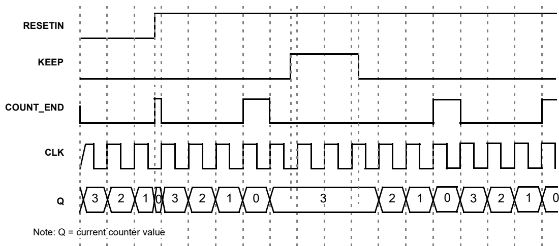
Figure 77: CNT/FSM Timing Diagram (Reset Rising Edge Mode, Oscillator is Forced On, UP=0) for Counter Data = 3
