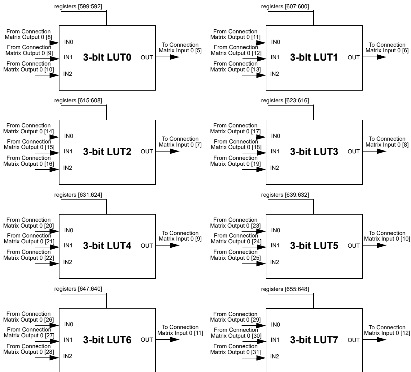
Figure 32: 3-bit LUTs
