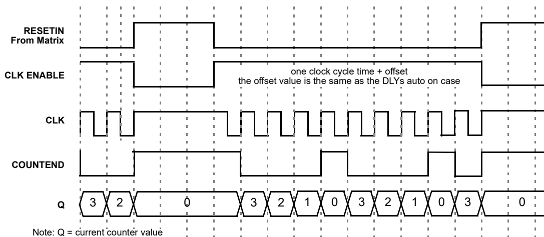
Figure 76: Timing (Reset High Level Mode, Oscillator is Autopowered on (Controlled by Reset)) for Count Data = 3
