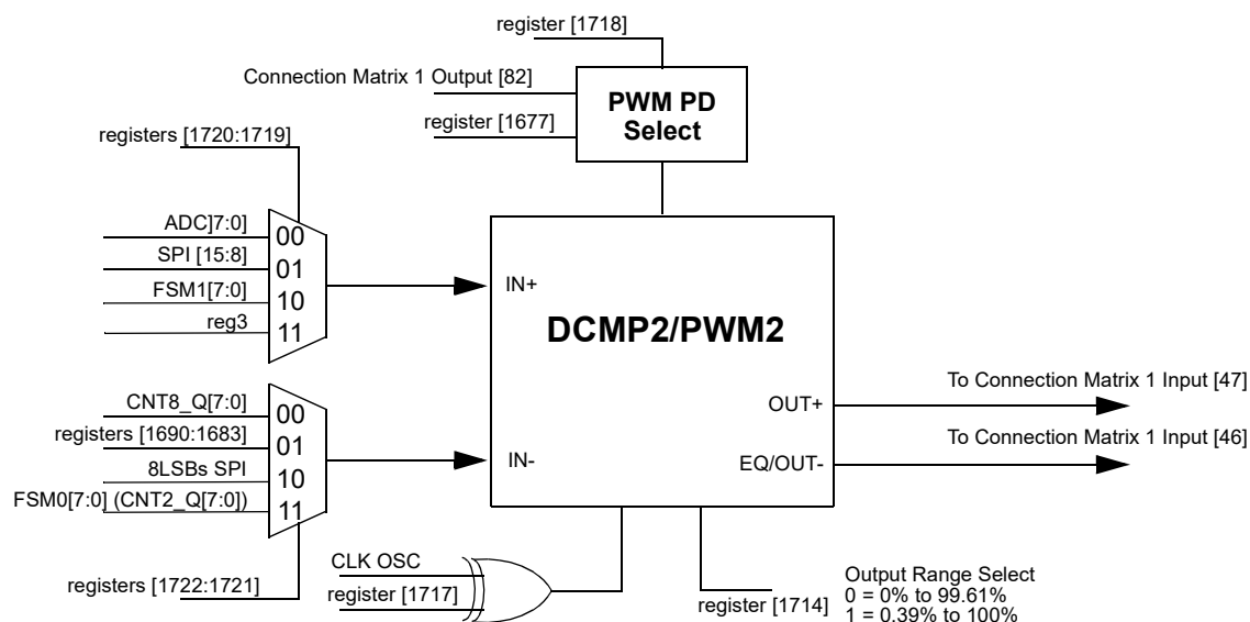
Figure 84: DCMP2/PWM2 Functional Diagram
