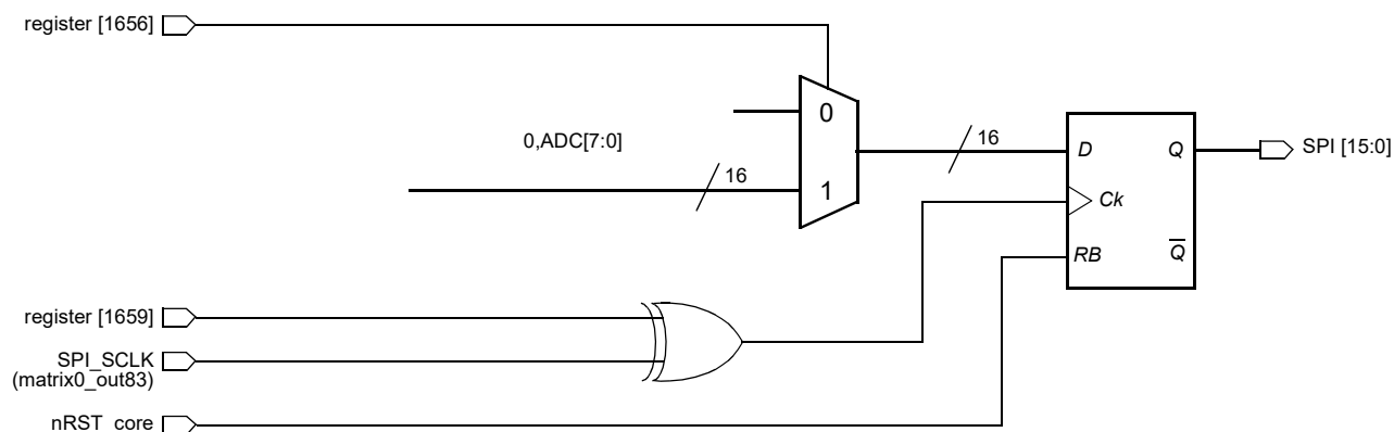
Figure 90: The SPI used as ADC data buffer diagram
