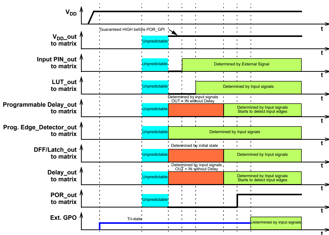
Figure 111: Internal Macrocell States during POR sequence
