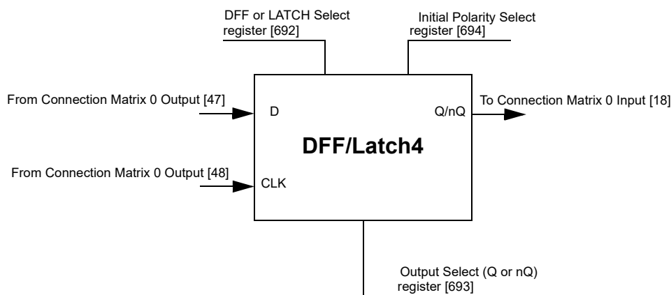
Figure 51: DFF/Latch4
