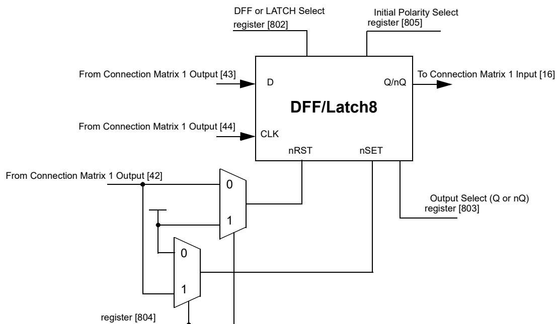
Figure 55: DFF/Latch8
