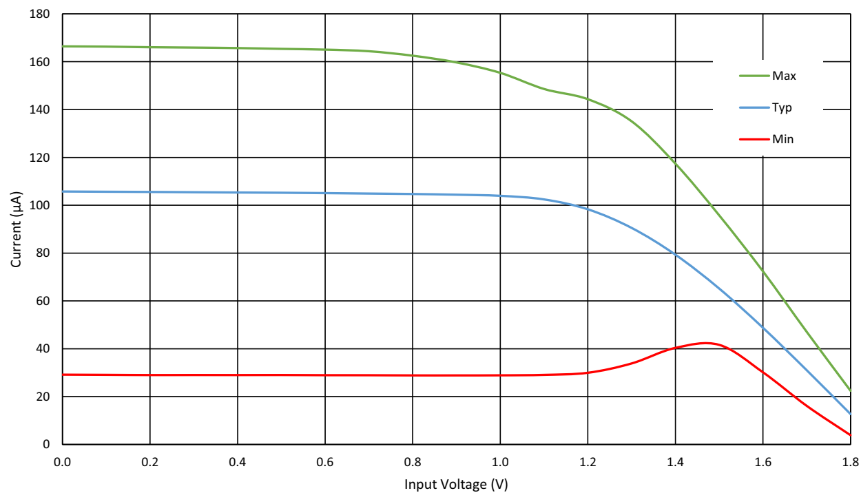
Figure 46: ACMP Input Current Source vs. Input Voltage at T = -40\text{ }^{\circ}\text{C} to 105\text{ }^{\circ}\text{C} , V_{DD} = 3.3\text{ V}
