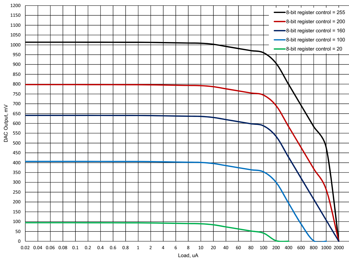
Figure 30: DAC Typical Load Regulation, T = 25^{\circ}\text{C} , V_{DD} = 3.3\text{ V}
