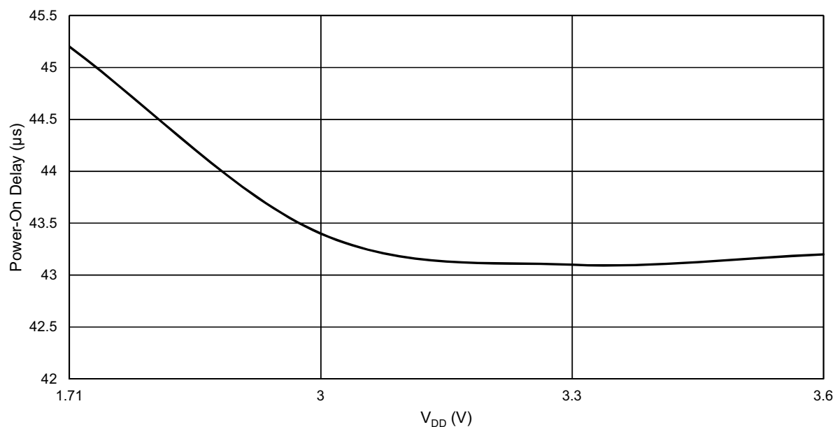
Figure 104: RC Oscillator Maximum Power-On Delay vs. V_{DD} at T = 25^{\circ}\text{C} , RC OSC = 25 kHz
