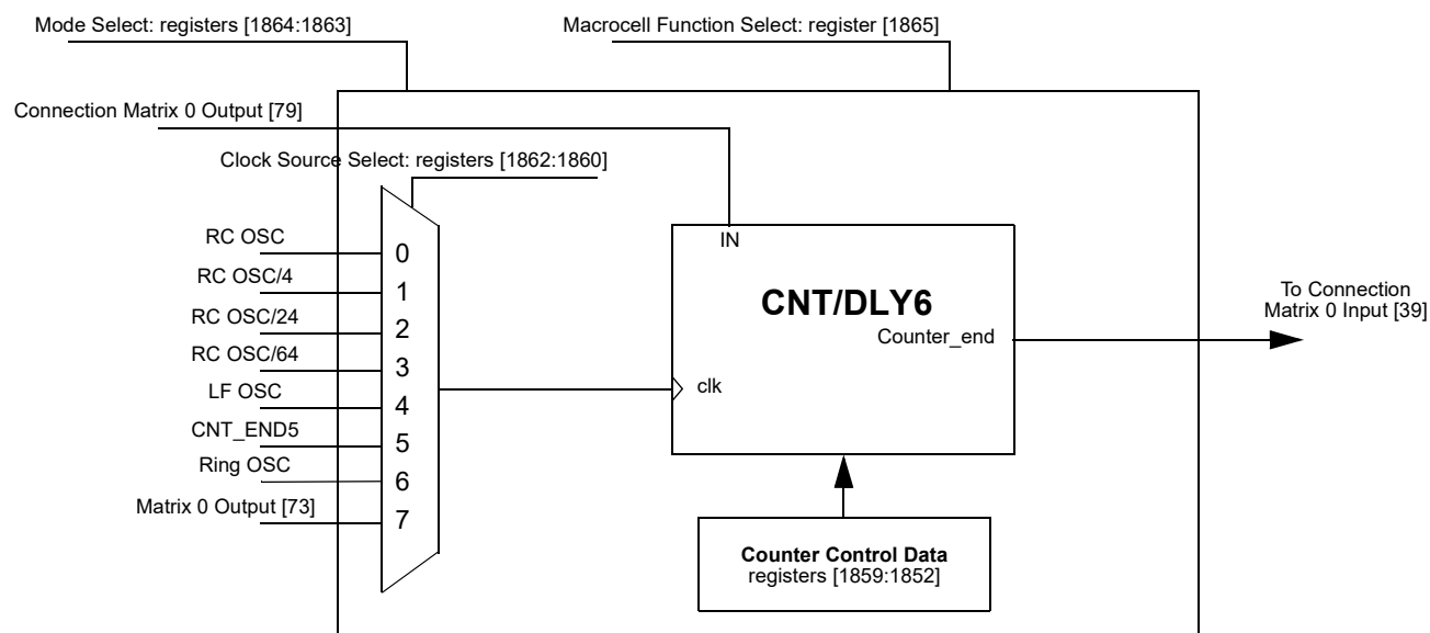
Figure 68: CNT/DLY6
