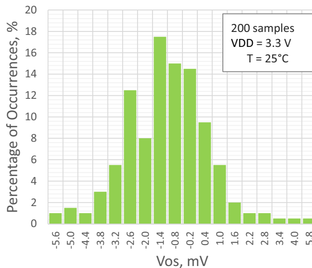
Figure 20: PGA Input Offset Distribution, Single-Ended Mode, G = 4
