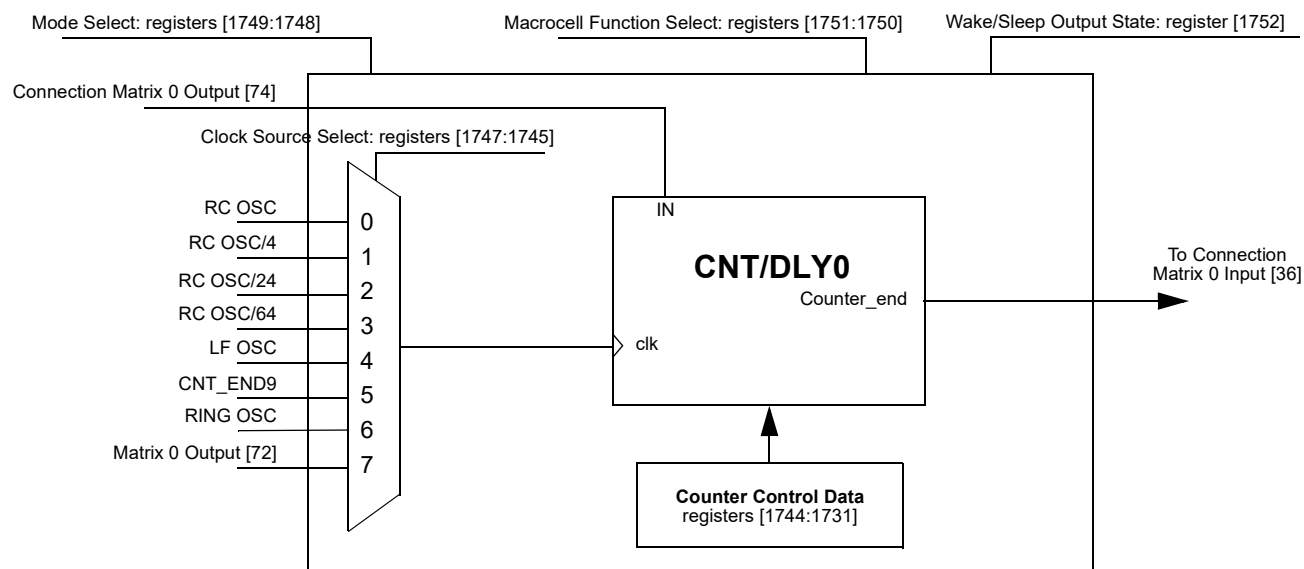
Figure 62: CNT/DLY0
