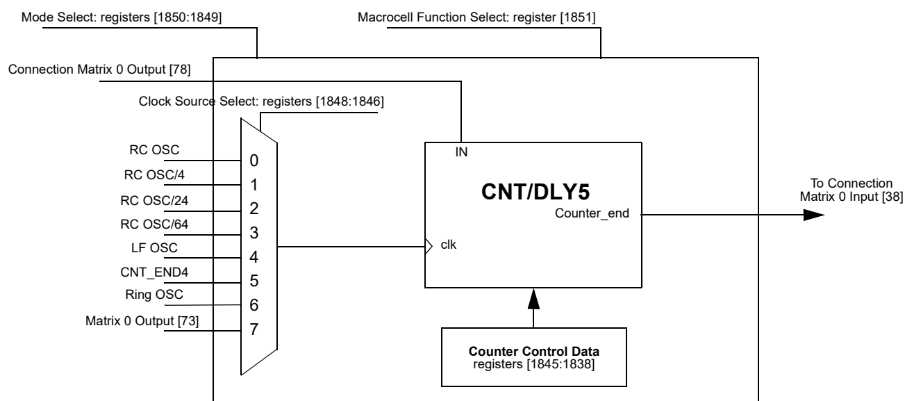
Figure 67: CNT/DLY5
