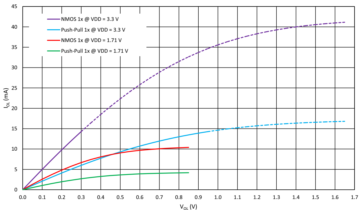
Figure 8: Typical Low Level Output Current vs. Low Level Output Voltage, 1x Drive at T = 25^\circ\text{C}
