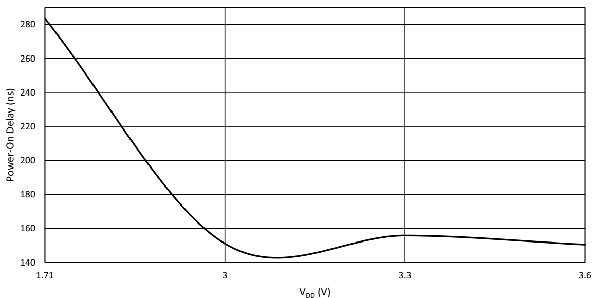
Figure 105: Ring Oscillator Maximum Power-On Delay vs. V_{DD} at T = 25^{\circ}\text{C} , \text{OSC} = 27 \text{ MHz}
