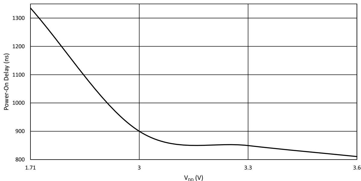
Figure 103: RC Oscillator Maximum Power-On Delay vs. V_{DD} at T = 25^{\circ}\text{C} , RC OSC = 2 MHz
