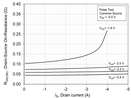
Figure 53. Drain-Source On-Resistance vs. Drain Current
