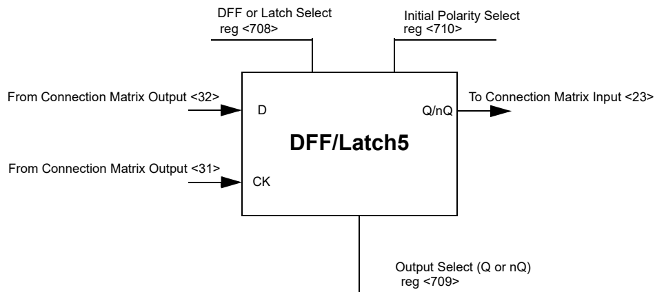
Figure 15. DFF/Latch5
