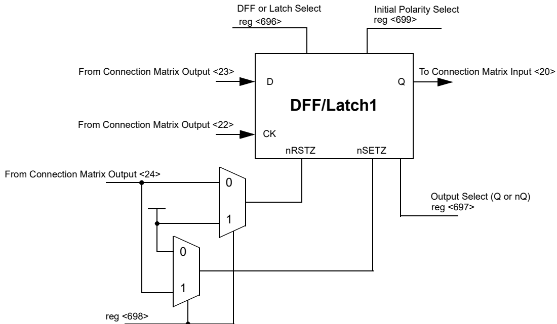
Figure 12. DFF/Latch1
