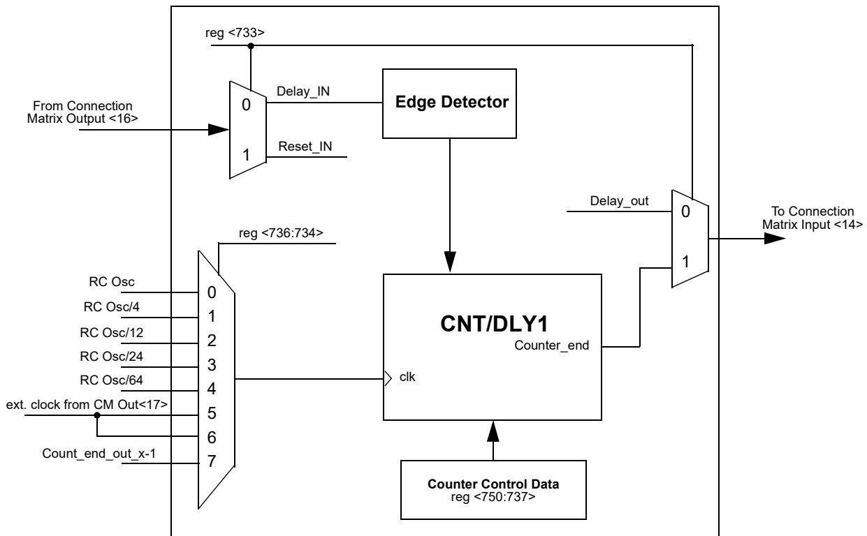
Figure 24. CNT/DLY1
