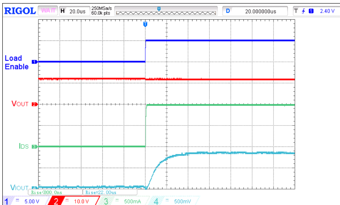
Figure 17. Typical I_{OUT} response time waveform for V_{IN} = 12 V, C_{LOAD} = 10 \mu F, R_{LOAD} = 12 \Omega C_{IOUT} = 0.18 nF, R_{IOUT} = 84.5 k \Omega , Load step 0 A to 1 A
