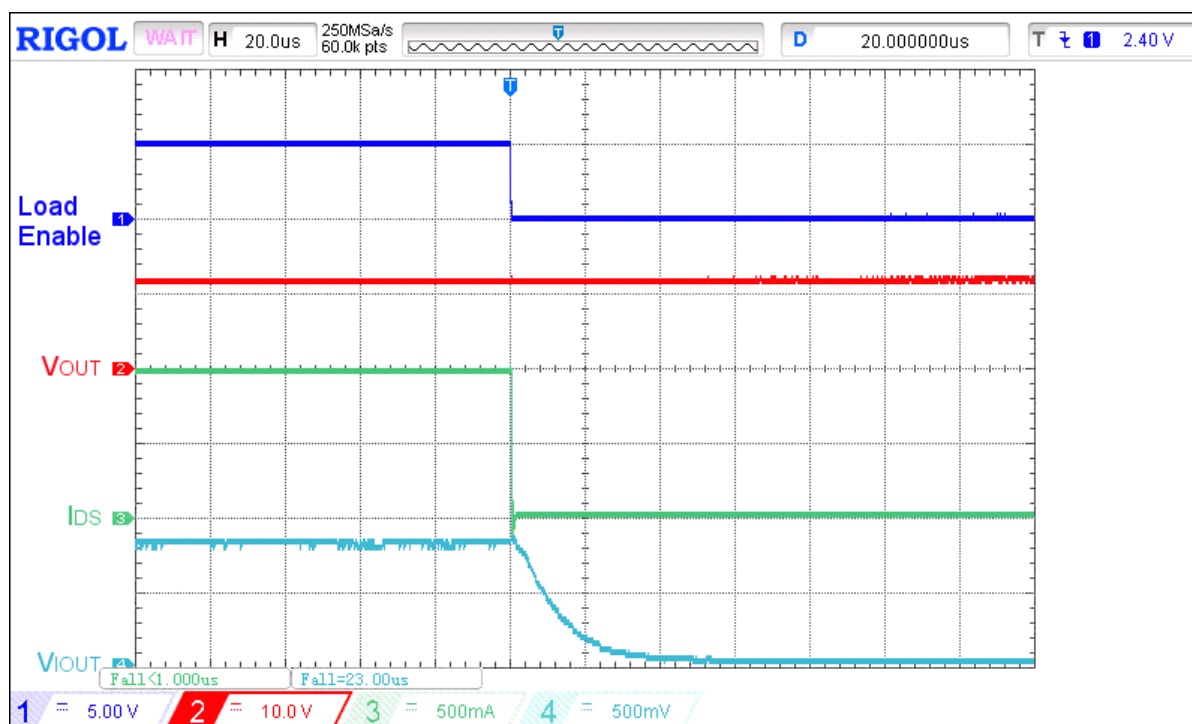
Figure 18. Typical I_{OUT} response time waveform for V_{IN} = 12 V, C_{LOAD} = 10 \mu F, R_{LOAD} = 12 \Omega C_{IOUT} = 0.18 nF, R_{IOUT} = 84.5 k \Omega , Load step 1 A to 0 A
