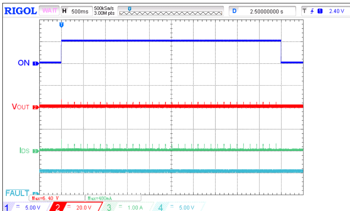
Figure 23. Typical SOA waveform during power up under heavy load for V_{IN} = 24 V, C_{LOAD} = 10 \mu F, R_{SET} = 30.1 k \Omega , R_{LOAD} = 12 \Omega
