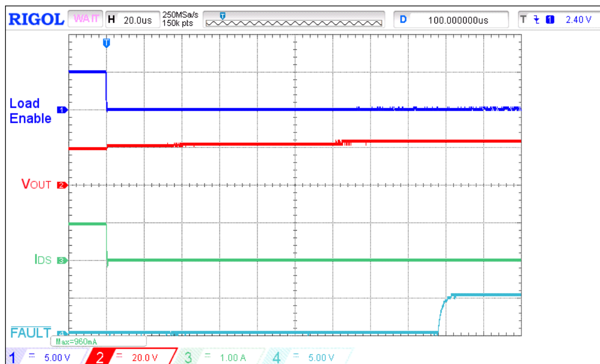
Figure 16. Typical \overline{\text{FAULT}} de-assertion waveform for V_{\text{IN}} = 24 \text{ V} , C_{\text{LOAD}} = 10 \mu\text{F} , I_{\text{ACL}} = 1 \text{ A} , R_{\text{SET}} = 91 \text{ k}\Omega , switch out 18.5 \Omega load
