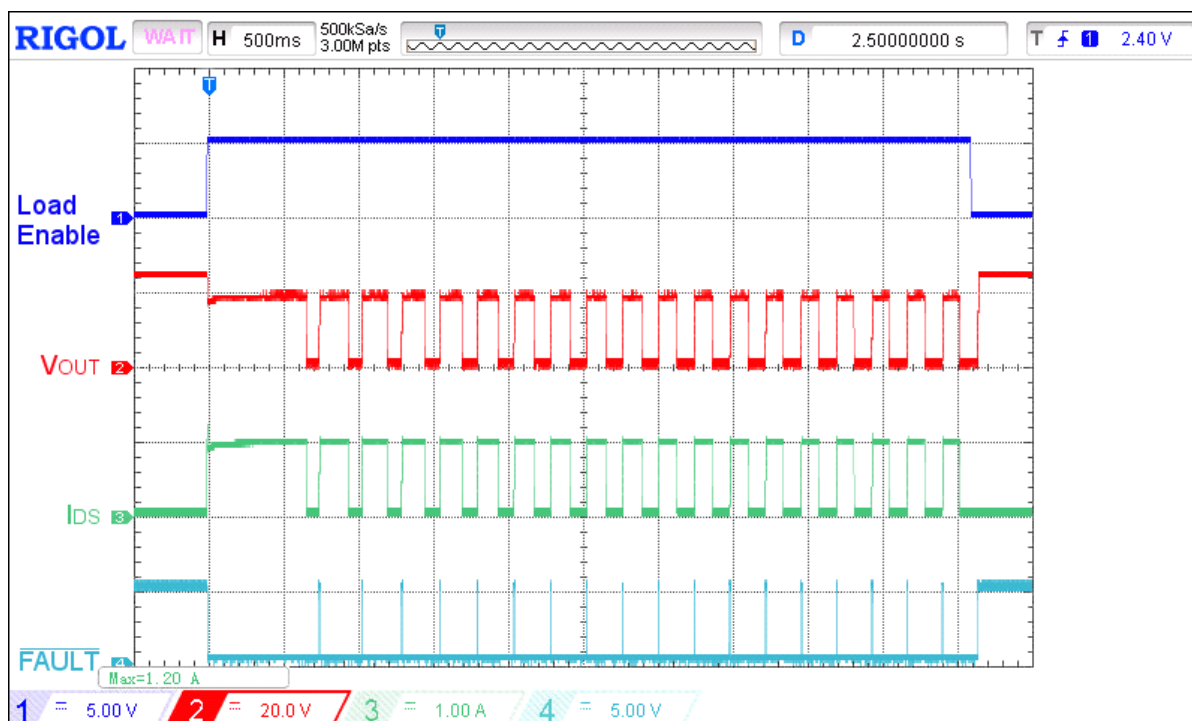
Figure 11. Typical ACL operation waveform for V_{IN} = 24 V, C_{LOAD} = 10 \mu F, I_{ACL} = 1 A, R_{SET} = 91 k \Omega
