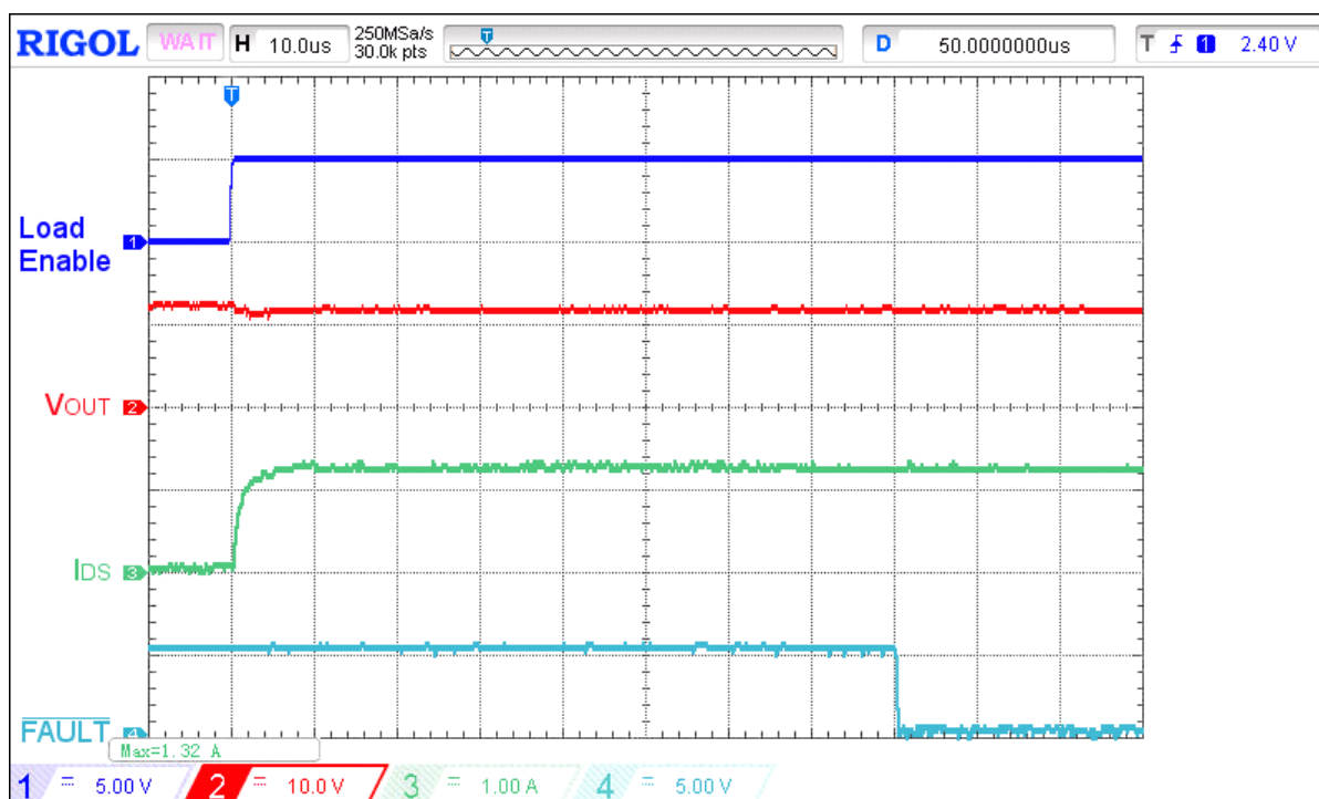
Figure 13. Typical FAULT assertion waveform for V_{IN} = 12 V, C_{LOAD} = 10 \mu F, I_{ACL} = 1 A, R_{SET} = 91 k \Omega , switch on 9 \Omega load
