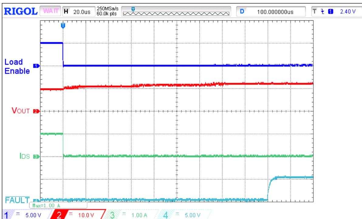
Figure 14. Typical FAULT de-assertion waveform for V_{IN} = 12 V, C_{LOAD} = 10 \mu F, I_{ACL} = 1 A, R_{SET} = 91 k \Omega , switch out 9 \Omega load
