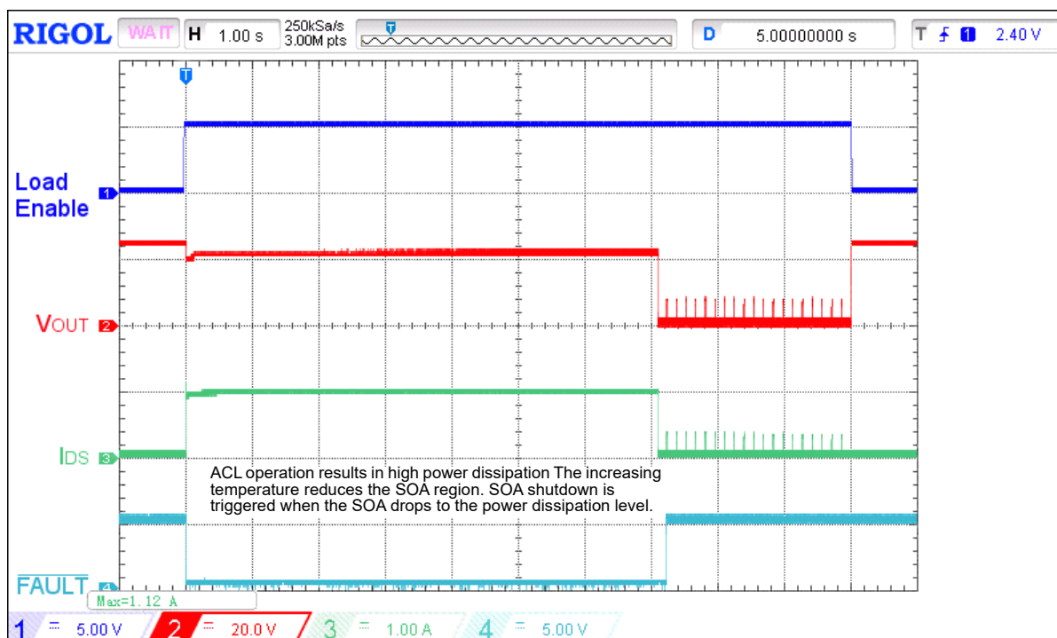
Figure 12. Thermally induced SOA shutdown for V_{IN} = 24 V, C_{LOAD} = 10 \mu F, R_{SET} = 91 k \Omega , I_{ACL} = 1 A, R_{LOAD} = 20 \Omega ,
