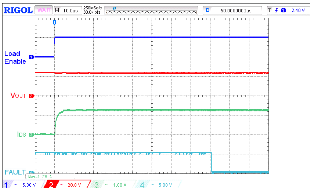
Figure 15. Typical \overline{\text{FAULT}} assertion waveform for V_{\text{IN}} = 24 \text{ V} , C_{\text{LOAD}} = 10 \mu\text{F} , I_{\text{ACL}} = 1 \text{ A} , R_{\text{SET}} = 91 \text{ k}\Omega , switch on 18.5 \Omega load
