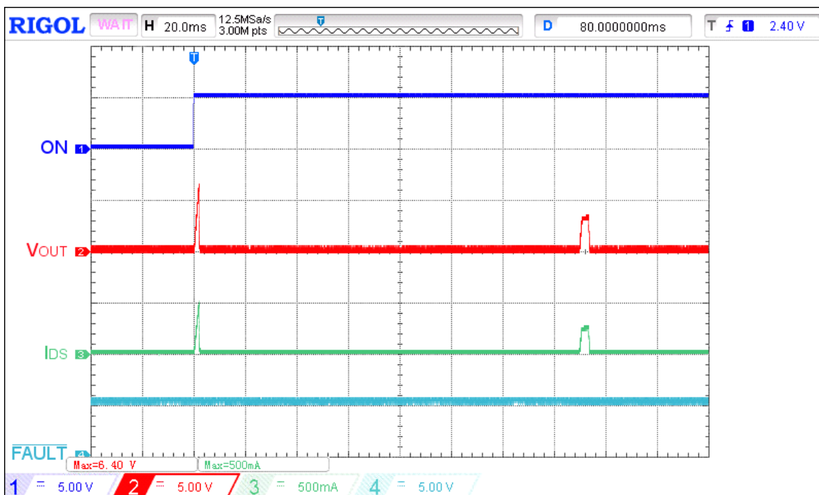
Figure 24. Extended typical SOA waveform during power up under heavy load for V_{IN} = 24 V, C_{LOAD} = 10 \mu F, R_{SET} = 30.1 k \Omega , R_{LOAD} = 12 \Omega
