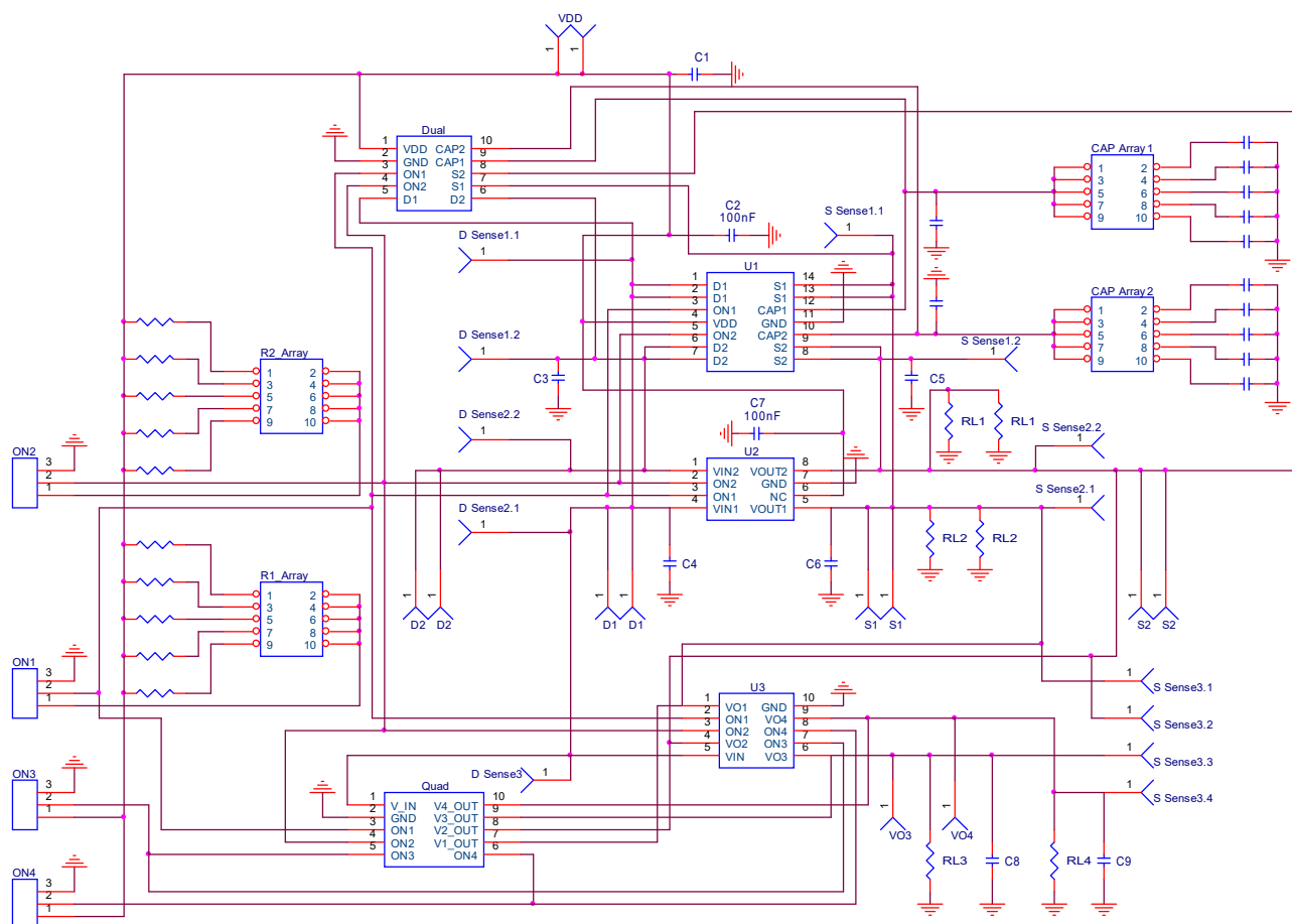
Figure 2. SLG59M1527V Evaluation Board Connection Circuit
