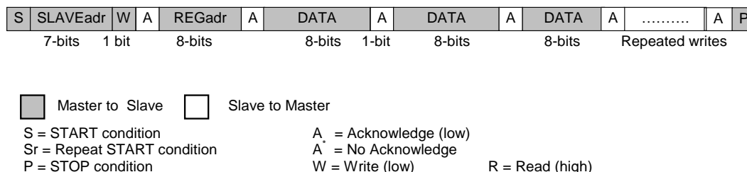
Figure 29: 2-WIRE Page Write (SDA Line)
