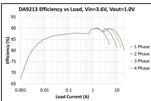
Figure 13: 1, 2, 3, and 4 Phase Modes
