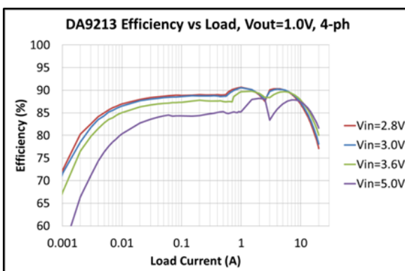
Figure 11: 4 Phase Auto-Mode, 0 to 20 A (Logarithmic)
