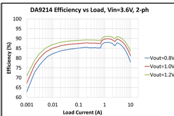
Figure 9: 2 Phase Auto-Mode, 0 to 10 A
