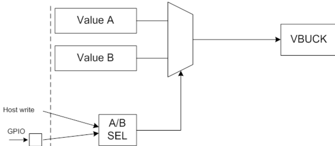
Figure 35: Concept of control of the buck's output voltage
